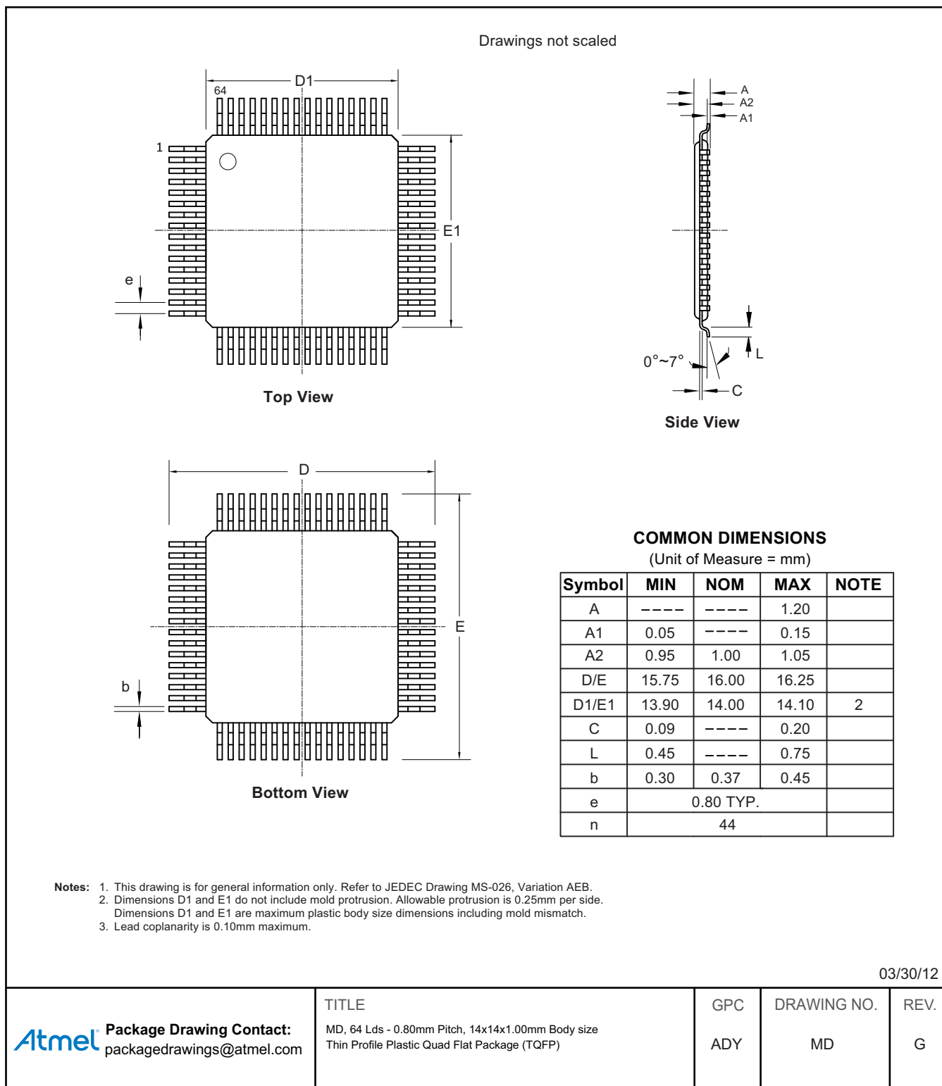
Figure 34-1. Package MD
