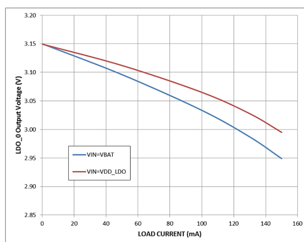
Figure 14: LDO_0 Dropout, V_{IN} = 3.15\text{ V} , V_{OUT} Setting = 3.15\text{ V}
