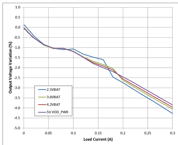
Figure 7: Buck Regulation, V_{OU} = 0.9 \text{ V}
