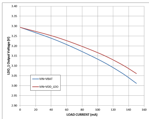
Figure 15: LDO_1 and LDO_2 Dropout, V_{IN} = 3.3\text{ V} , V_{OUT} Setting = 3.3\text{ V}
