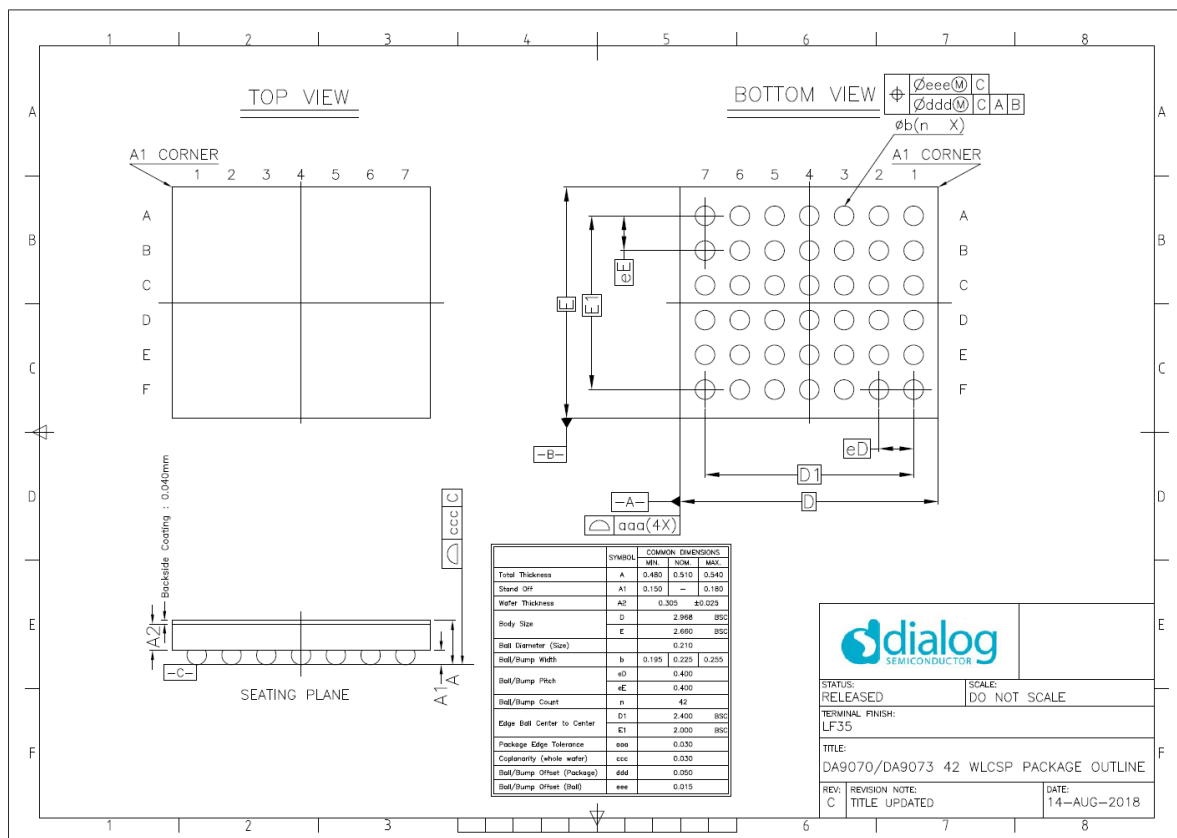
Figure 44: WLCSP-42 Package Outline Drawing
