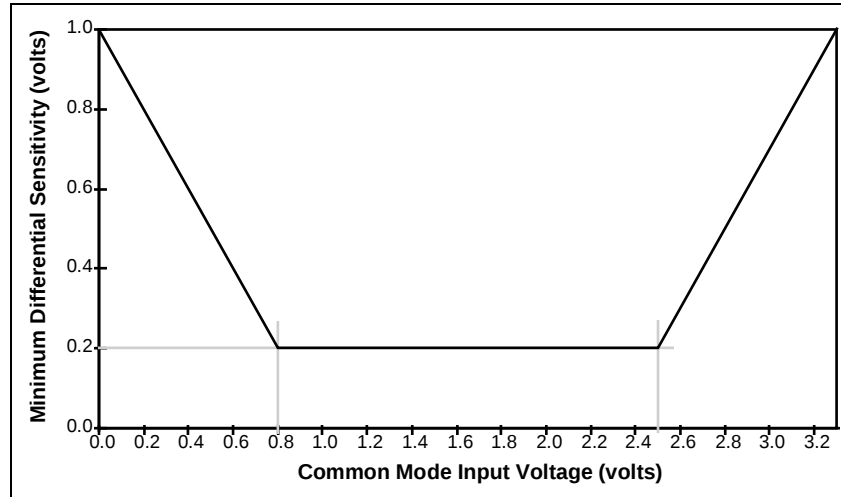
FIGURE 4 - DIFFERENTIAL INPUT SENSITIVITY OVER ENTIRE COMMON MODE RANGE
