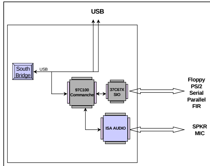
TYPICAL PC MOTHERBOARD APPLICATION
