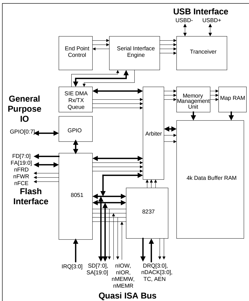
FIGURE 2 - BLOCK DIAGRAM
