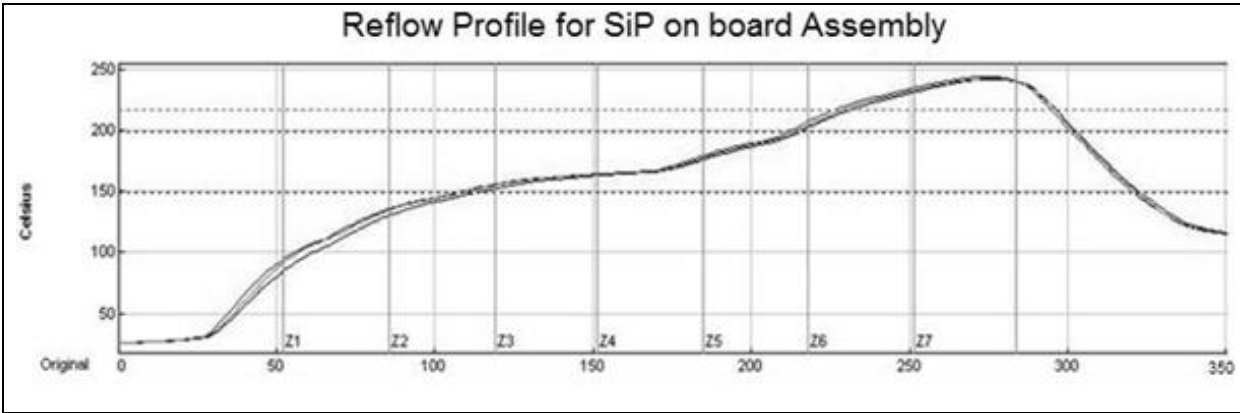
Figure 8.3-2 Profile Suggestion for N9H30 series
