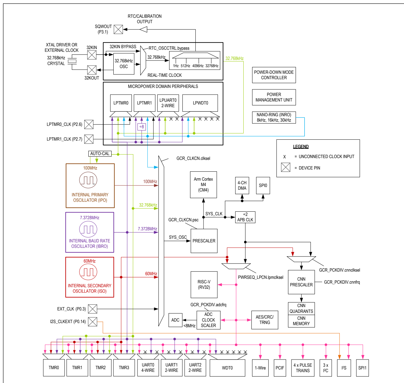
Figure 7. Clocking Scheme Diagram
