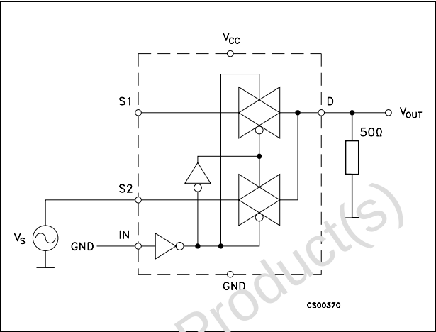
Figure 7. Channel-to-channel crosstalk
