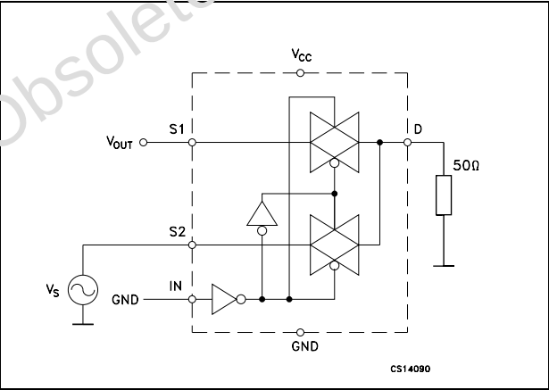
Figure 7. Channel-to-channel crosstalk
