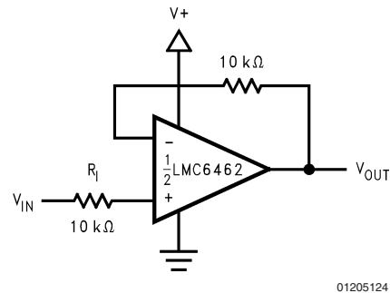
FIGURE 18. Half-Wave Rectifier with Input Current Protection ( R_1 )
