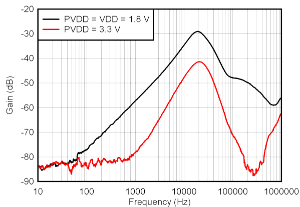
Figure 6-48. Reference AC PSRR vs frequency
