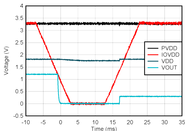
Figure 6-32. DAC IOVDD Supply Collapse Response, RANGE = 1
