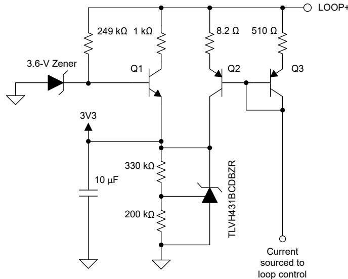
Figure 8-4. Start-Up Circuit
