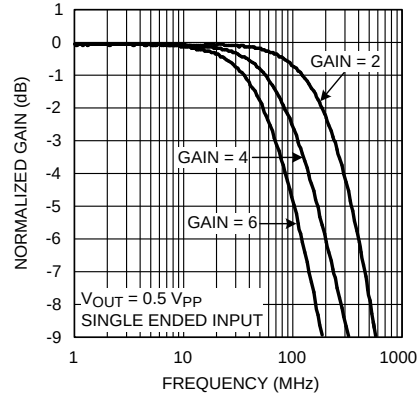
Figure 4. Frequency Response vs Gain
