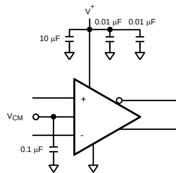
Figure 24. Single Supply Bypassing Capacitors
