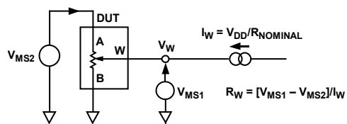
Figure 29. Wiper Resistance
