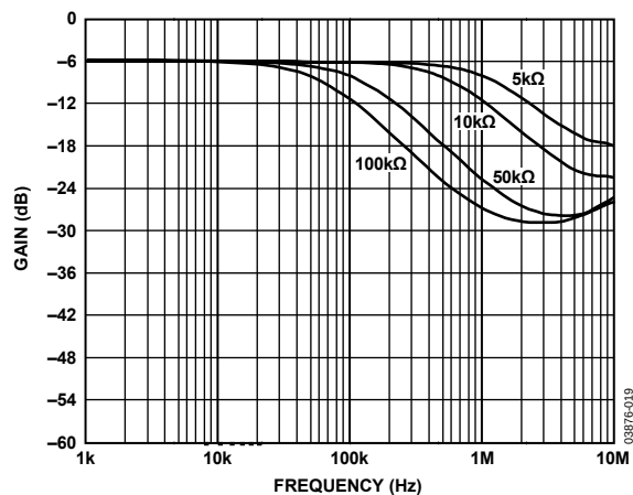
Figure 21. -3 \text{ dB} Bandwidth @ Code = 0x80
