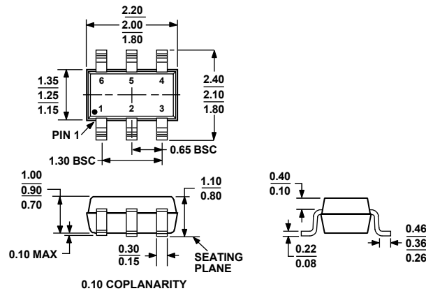
Figure 43. 6-Lead Thin Shrink Small Outline Transistor Package [SC70] (KS-6)
