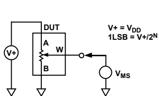
Figure 27. Potentiometer Divider Nonlinearity Error (INL, DNL)
