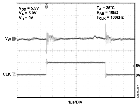
Figure 24. Digital Feedthrough
