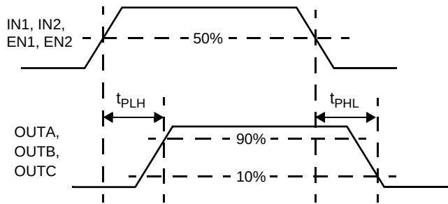
Figure 4. t PLH , t PHL , and t PZH Timing
