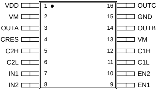
Figure 3. 17517 Pin Connections
