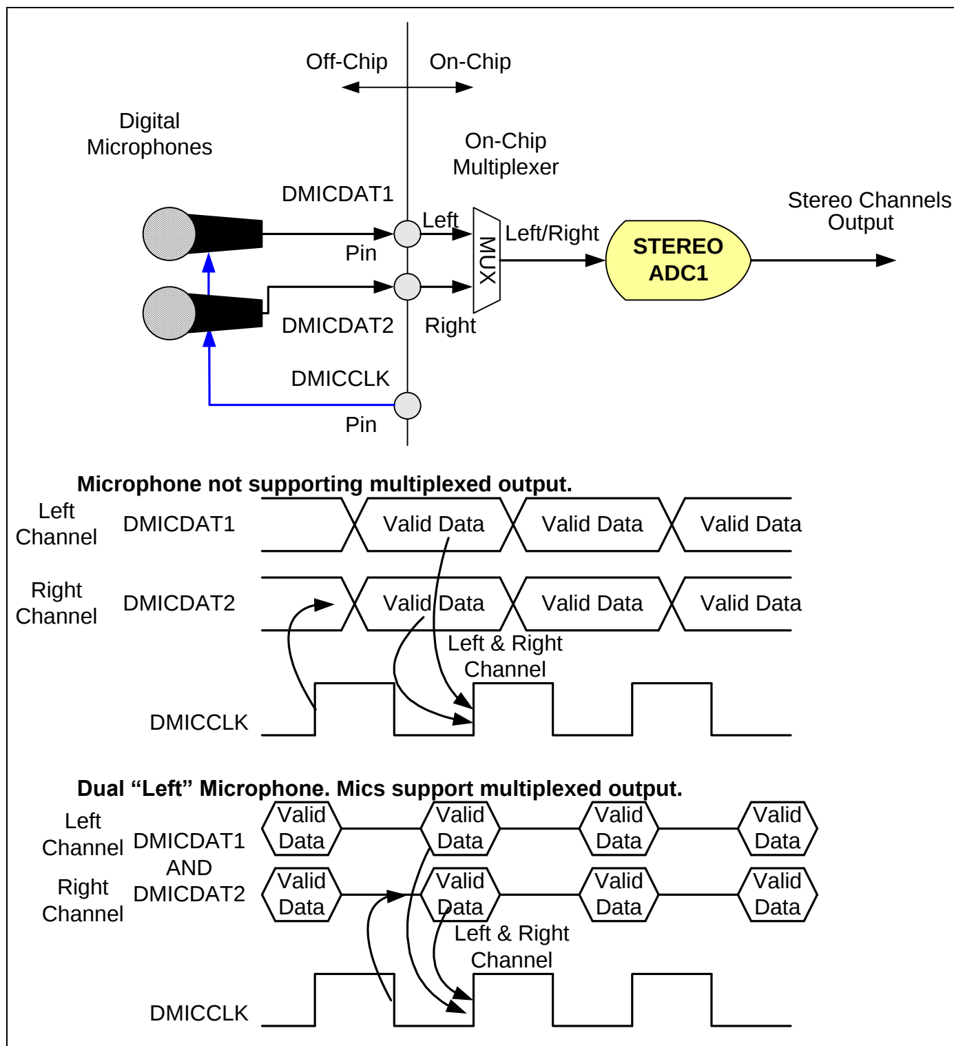
Figure 6 –Stereo Digital Microphone (Mode 3)
