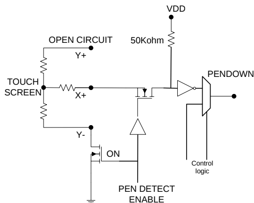
PEN-DOWN DETECTION Function Block Diagram.
