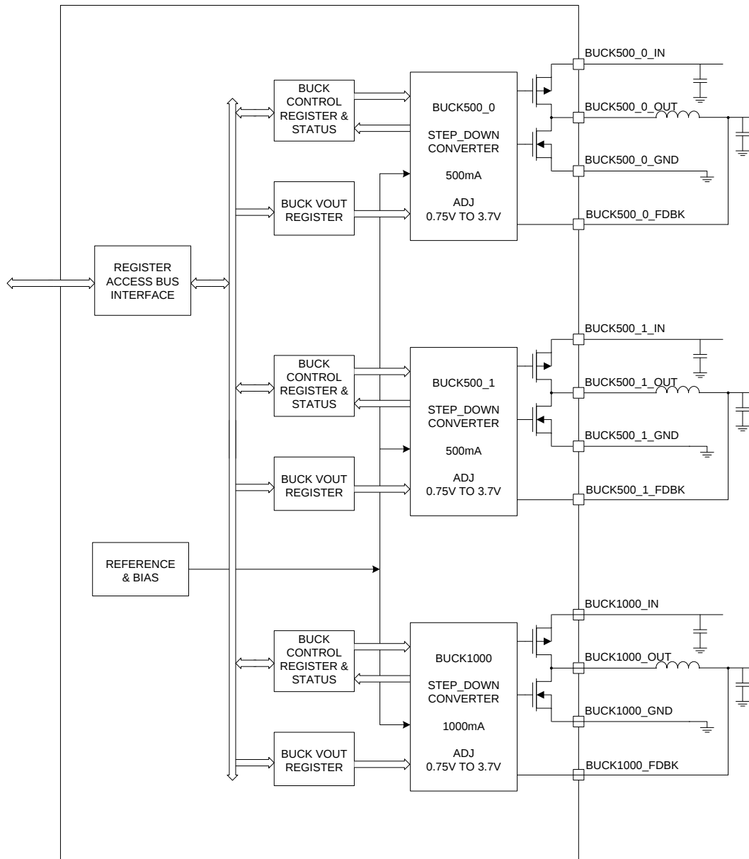
Figure 16 – BUCK500 / BUCK1000 Block Diagram
