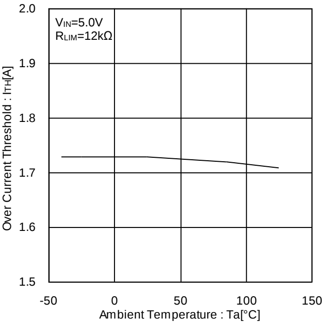
Figure 19. Over Current Threshold 3 vs Ambient Temperature
