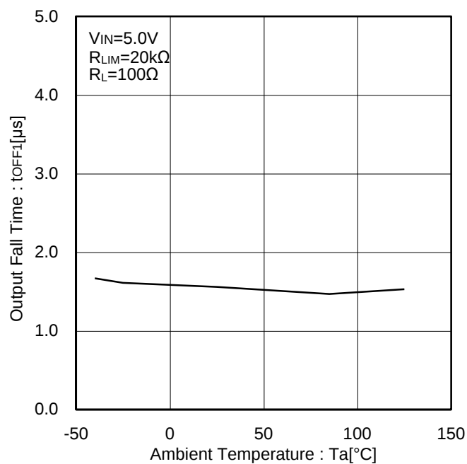
Figure 29. Output Fall Time vs Ambient Temperature
