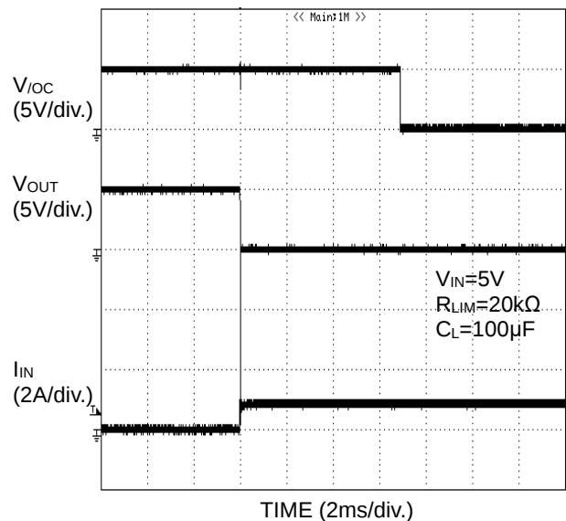
TIME (2ms/div.) Figure 46. Over Current Response 0Ω Load Connected At Enable
