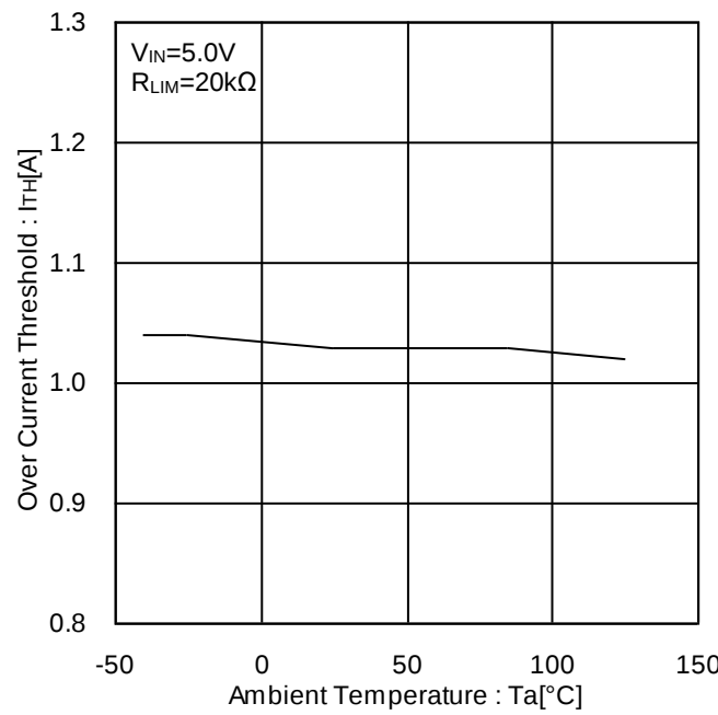
Figure 17. Over Current Threshold 2 vs Ambient Temperature
