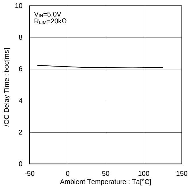
Figure 33. /OC Delay Time vs Ambient Temperature
