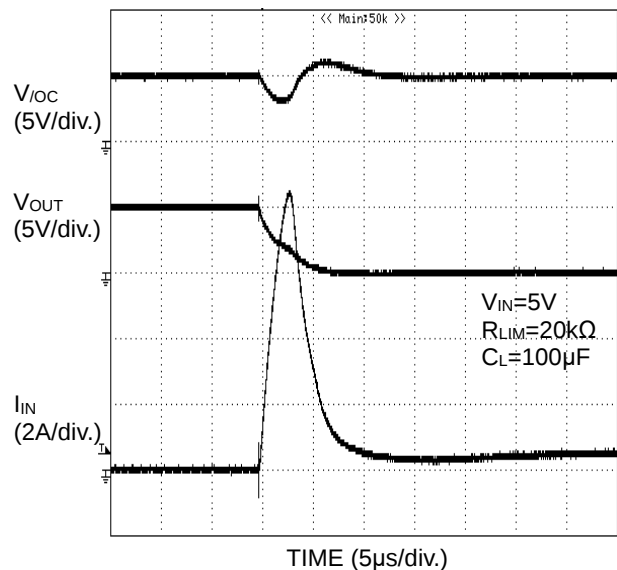
TIME (5μs/div.) Figure 47. Over Current Response 0Ω Load Connected At Enable
