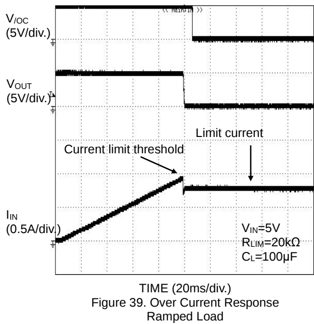
Figure 39. Over Current Response Ramped Load
