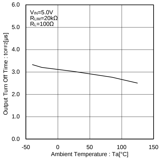
Figure 31. Output Turn Off Time vs Ambient Temperature
