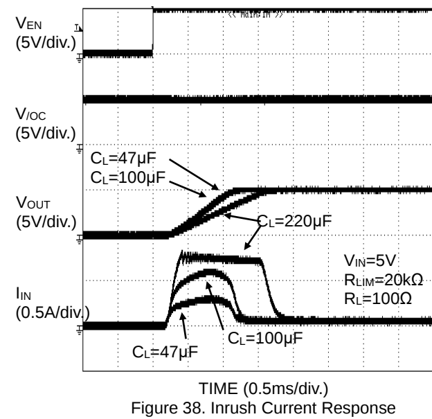
Figure 38. Inrush Current Response
