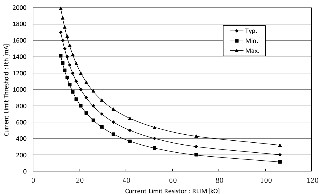
Figure 51. I_{TH} vs. R_{LIM}
