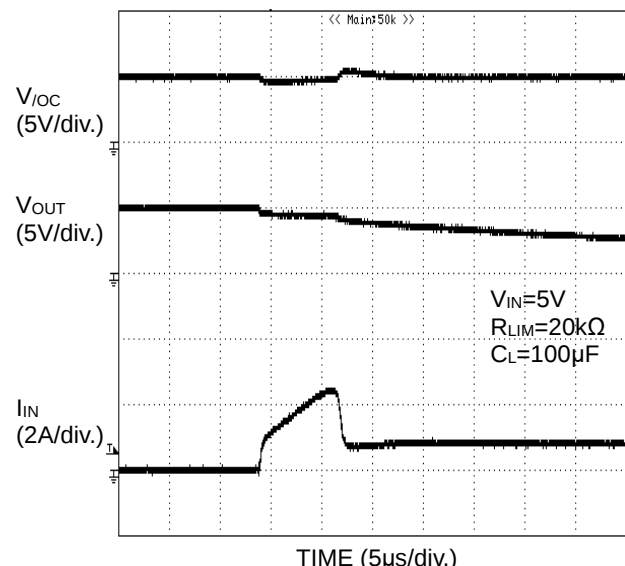
TIME (5μs/div.) Figure 45. Over Current Response 1Ω Load Connected At Enable
