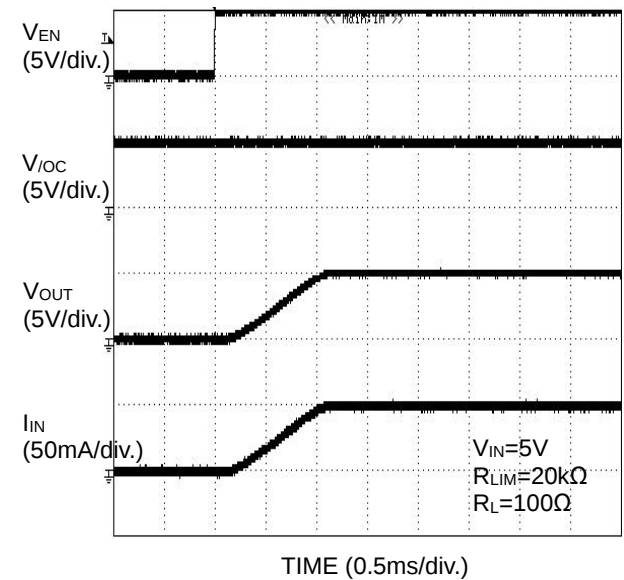
Figure 36. Output Rise Characteristic
