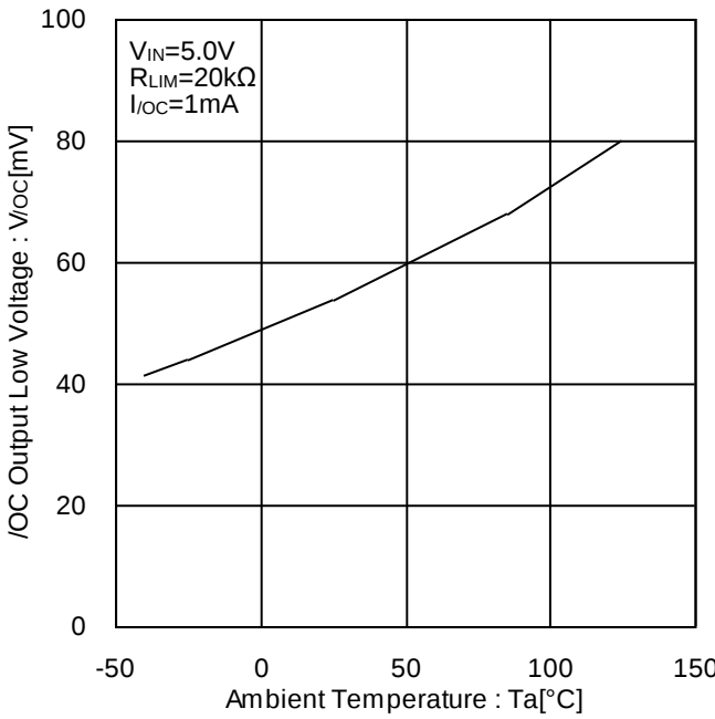
Figure 21. /OC Output Low Voltage vs Ambient Temperature
