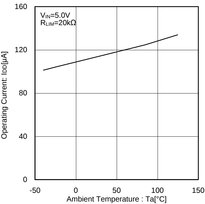
Figure 7. Operating Current vs Ambient Temperature (EN Enable)
