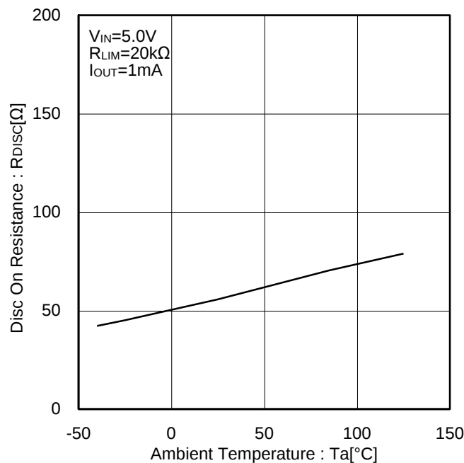
Figure 35. Discharge On Resistance vs Ambient Temperature
