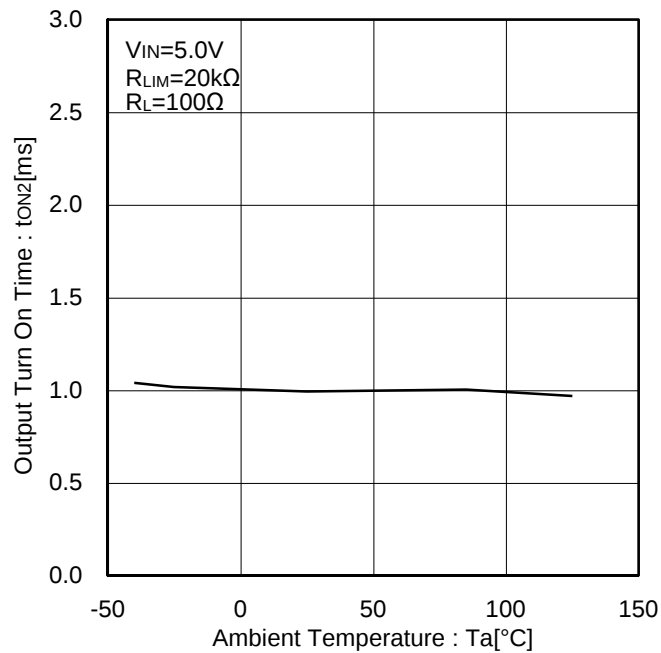
Figure 27. Output Turn On Time vs Ambient Temperature
