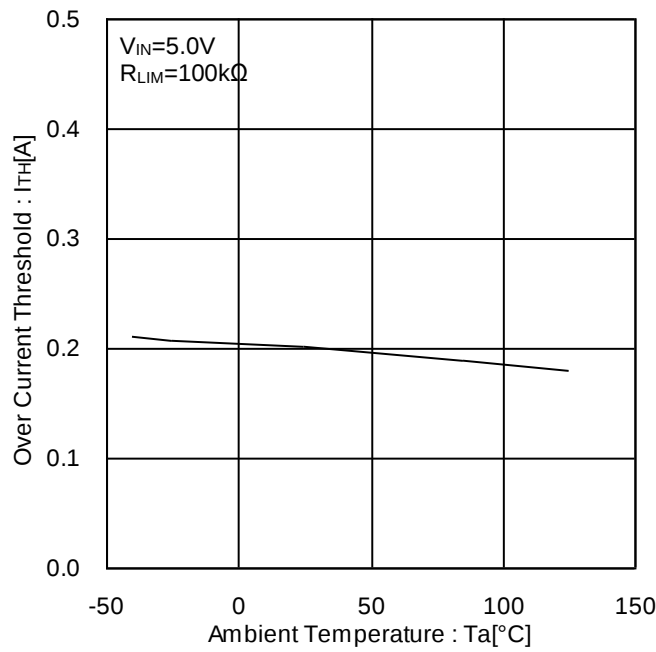
Figure 15. Over Current Threshold 1 vs Ambient Temperature
