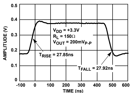
FIGURE 12. SMALL SIGNAL STEP RESPONSE
