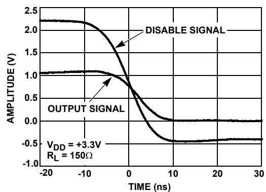
FIGURE 14. DISABLE TIME
