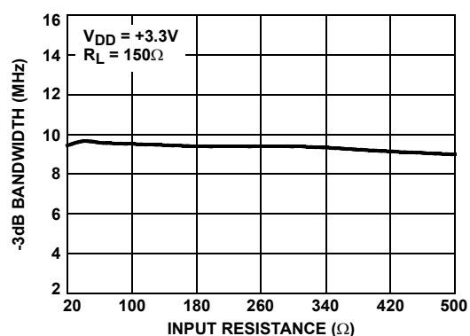
FIGURE 18. -3dB BANDWIDTH vs INPUT RESISTANCE
