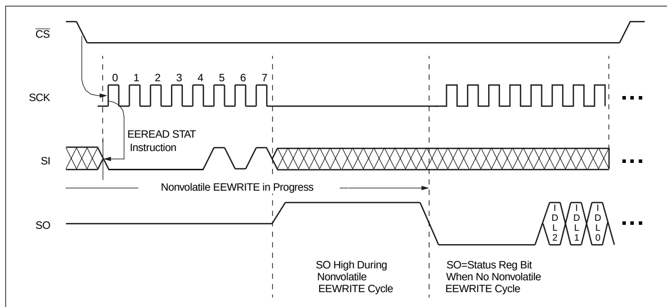
Figure 14. EEPROM Read Status (EEREAD STAT) Operation Sequence
