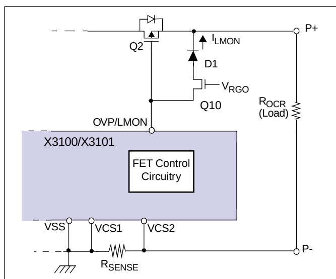
Figure 7. Over-Current Protection
