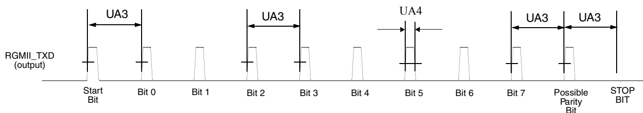
Figure 73. UART IrDA Mode Transmit Timing Diagram
