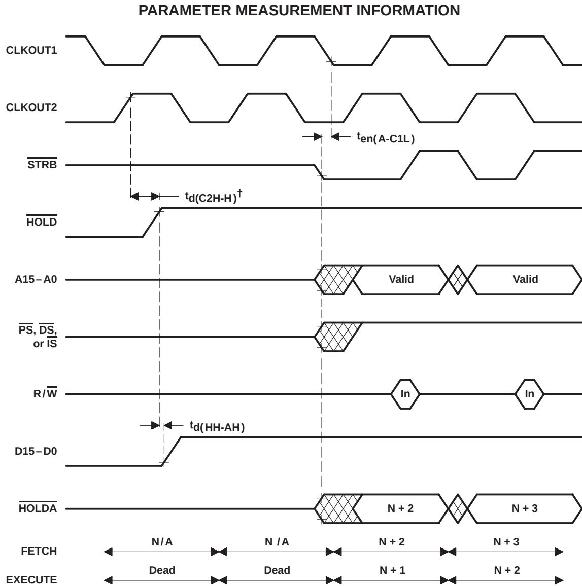
Figure 17. \overline{\text{HOLD}} Timing (Part B)
