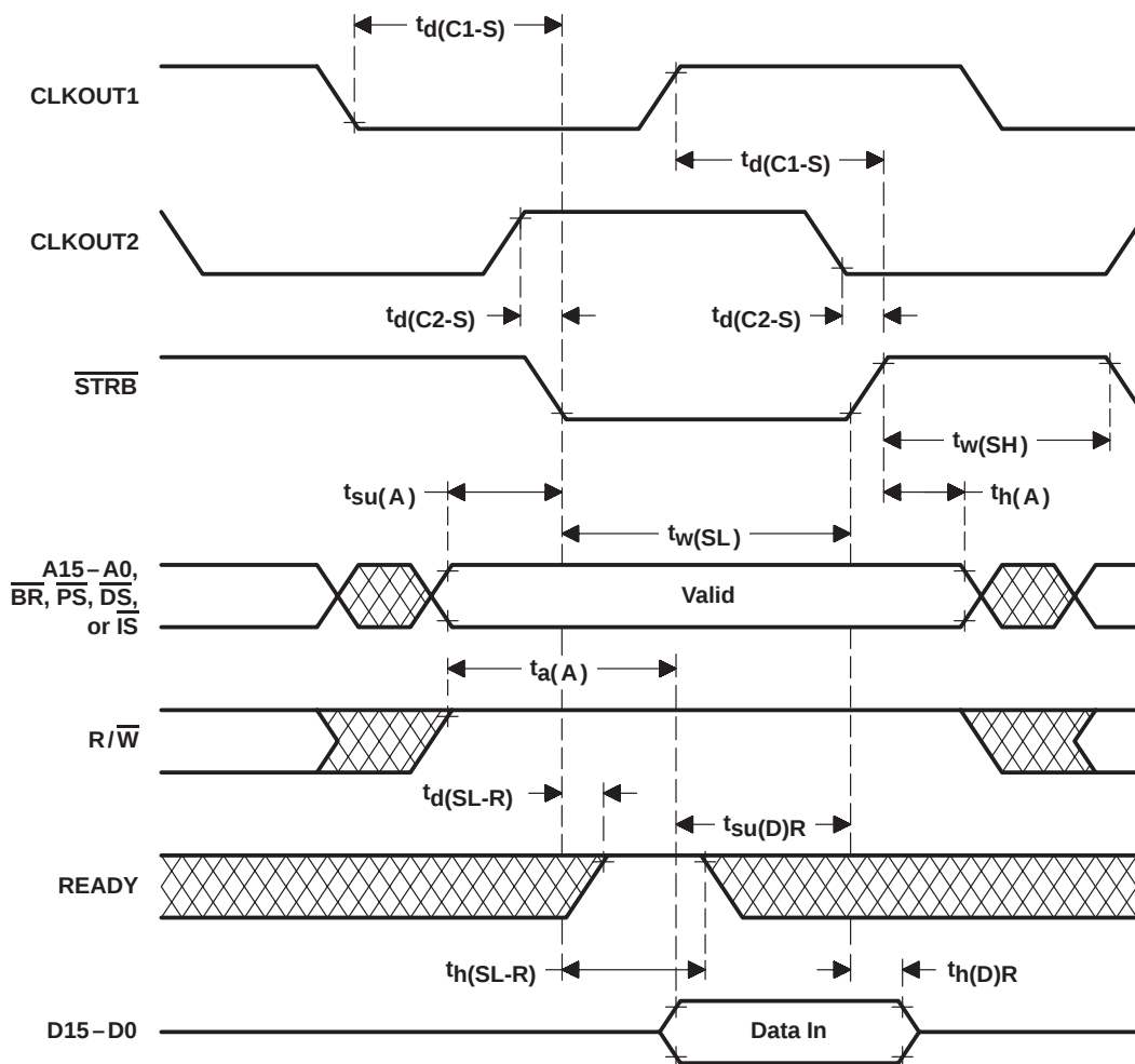
Figure 7. Memory-Read-Cycle Timing
