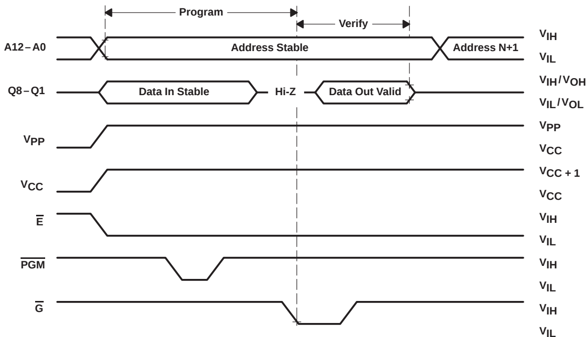
Figure 24. Programming Timing
