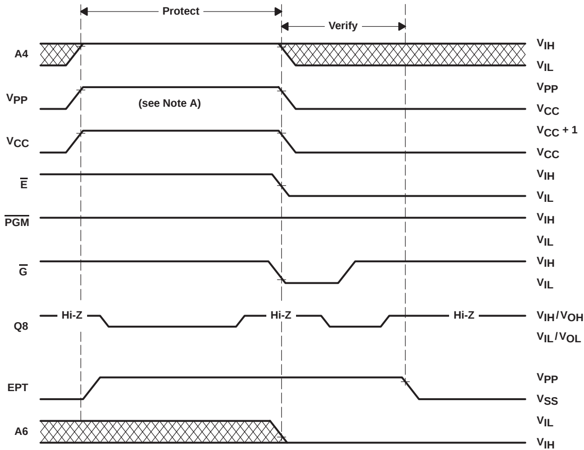
Figure 27. EPROM-Protection Timing
