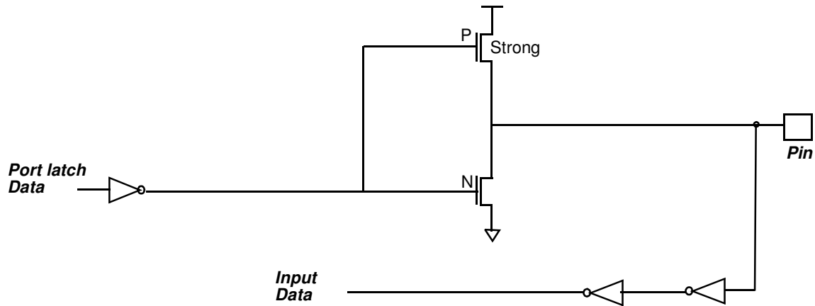
Figure 13. Push-Pull Output
