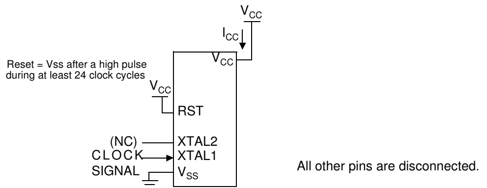
Figure 39. Operating I_{CC} Test Condition
