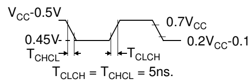
Figure 42. Clock Signal Waveform for I_{CC} Tests in Active and Idle Modes
