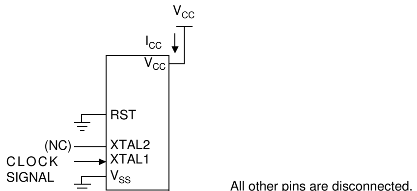
Figure 38. I_{CC} Test Condition, under reset
