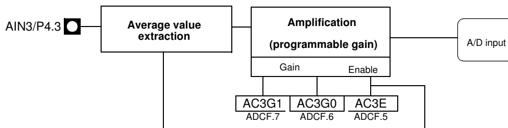
Figure 28. Channel 3 Amplifier
