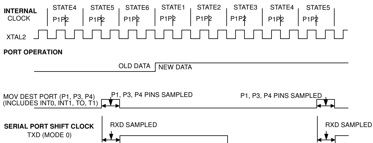
Figure 46. Clock Waveforms
