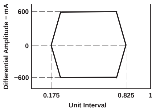
Figure 18. Transmit Template
