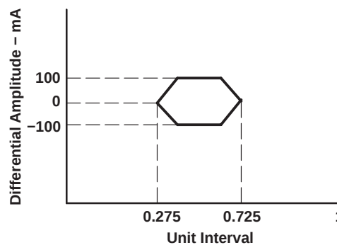
Figure 19. Receive Template
