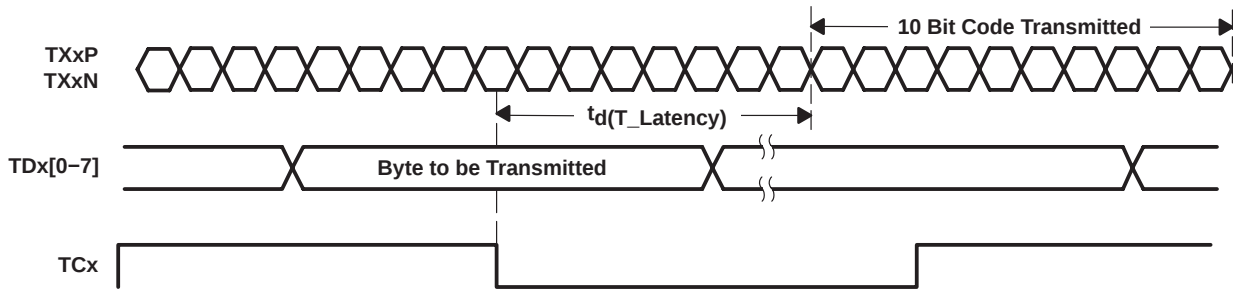
Figure 5. Transmitter Latency
