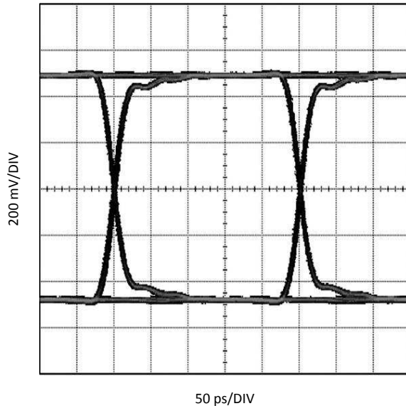
Figure 12. Eye Measured at Point (A)
