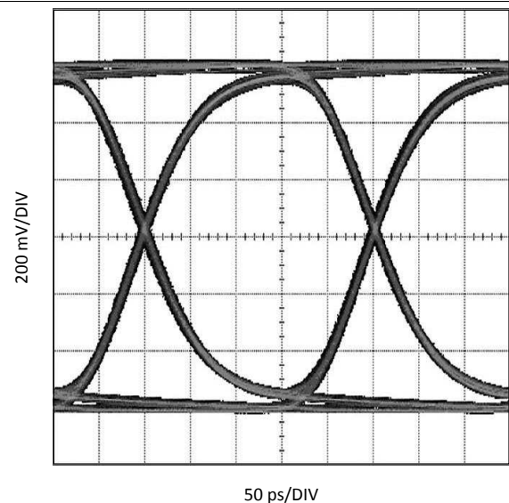
Figure 14. Eye Measured at Point (C), Pre-Emph = 0 dB
