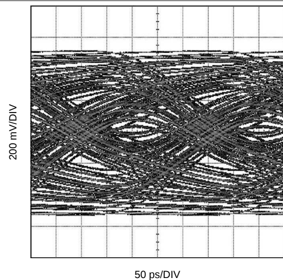
Figure 15. Eye Measured at Point (D), Pre-Emph = 0 dB
