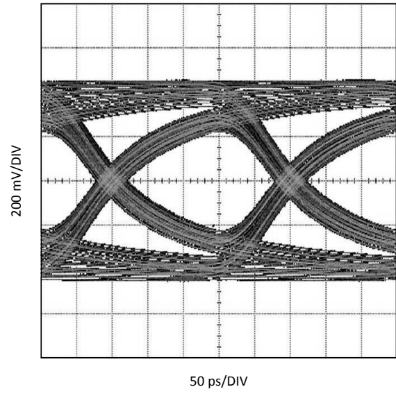
Figure 13. Eye Measured at Point (B)
