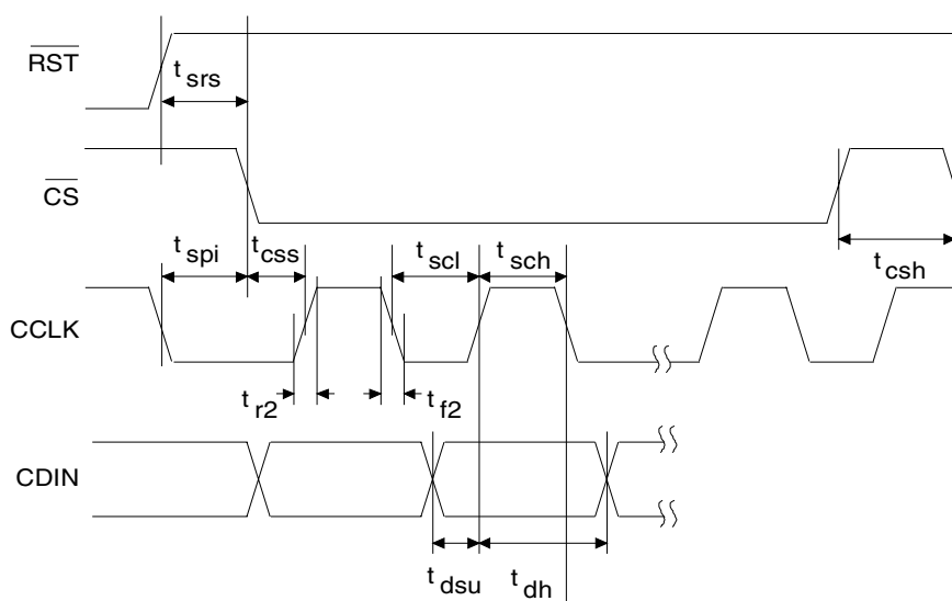
Figure 2. SPI Control Port Timing
