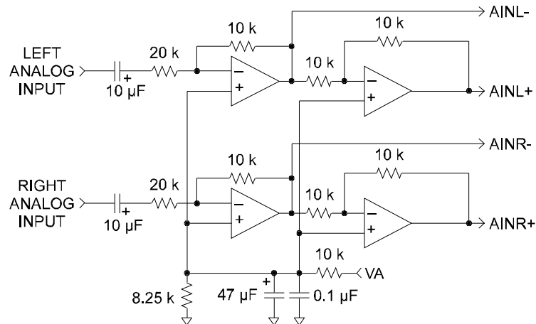
Figure 12. Optional Input Buffer
