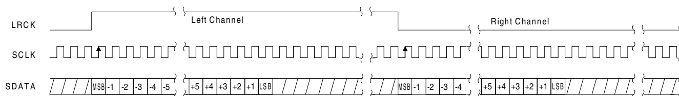
Figure 8. Serial Audio Format 0 (I²S)
