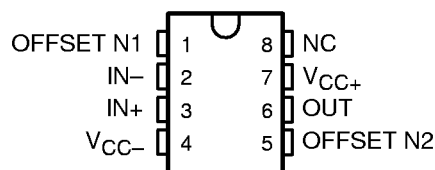
TL061 . . . U PACKAGE (TOP VIEW)
