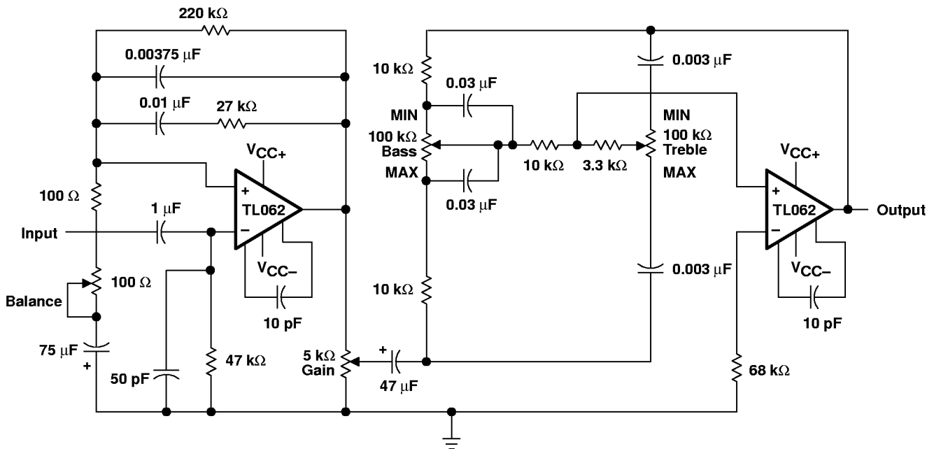
Figure 27. IC Preamplifier
