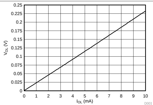
Figure 5. I_{OL} vs V_{OL}
