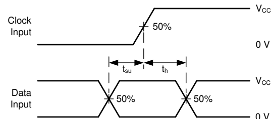
Figure 6-3. Voltage Waveforms, Standard CMOS Inputs Setup and Hold Times
