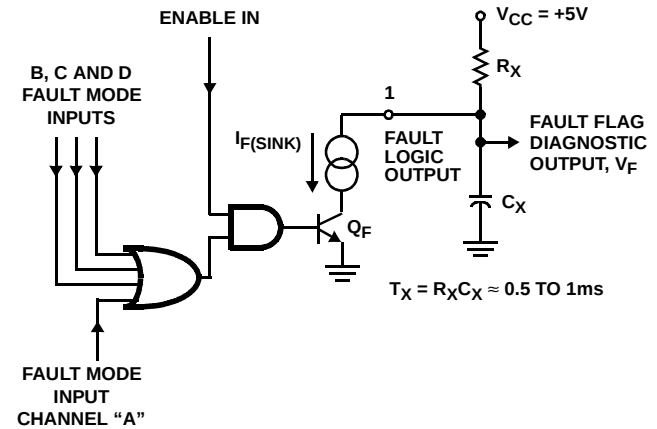
FIGURE 2. EXTERNAL FAULT OUTPUT CIRCUIT AND I_F(SINK) AS FAULT SINK PULLDOWN CURRENT, WHICH IS ACTIVATED BY TRANSISTOR, Q_F , WHEN A FAULT EXISTS
