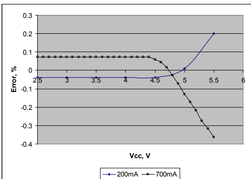
SP7619A Line Regulation at 25°C
