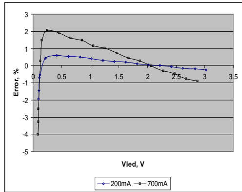
SP7619A Load Regulation at 25°C
