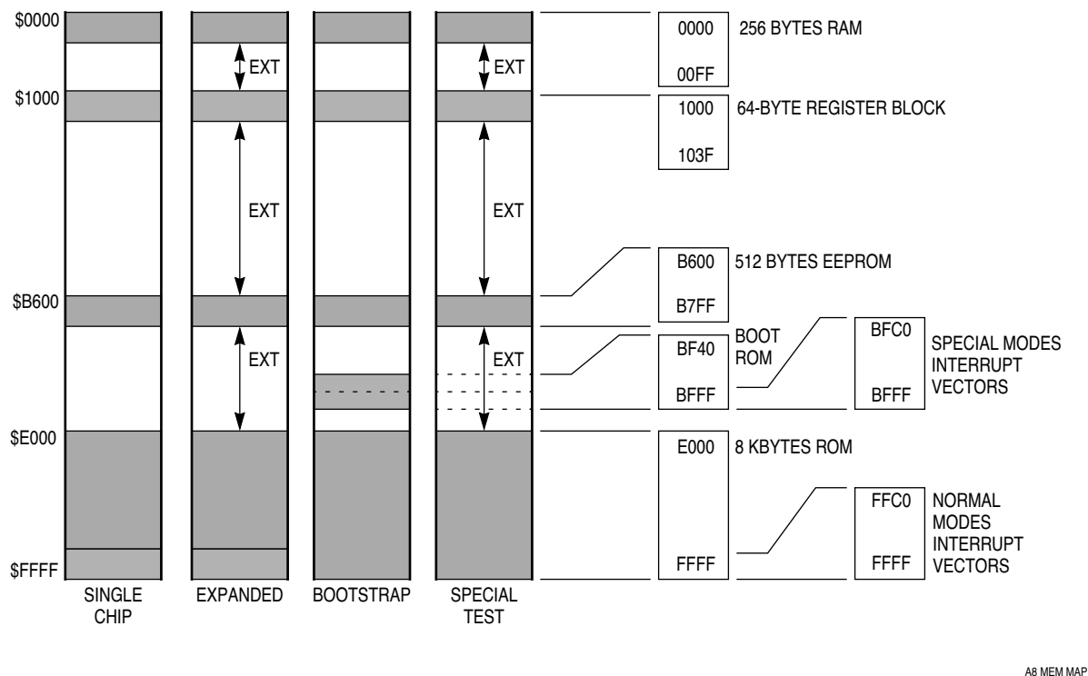
Figure 3-1 Memory Maps
