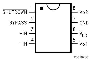
Top View Order Number LM4890MM See NS Package Number MUA08A
