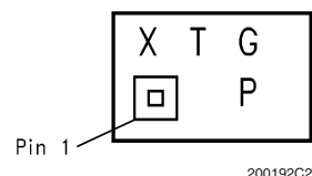
Top View X - Date Code T - Die Traceability G - Boomer Family P - LM4890IBL
