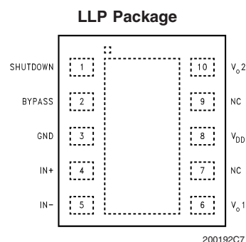
Top View Order Number LM4890LD See NS Package Number LDA10B
