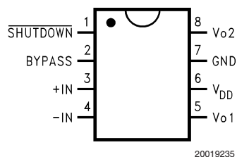
Top View Order Number LM4890M See NS Package Number M08A
