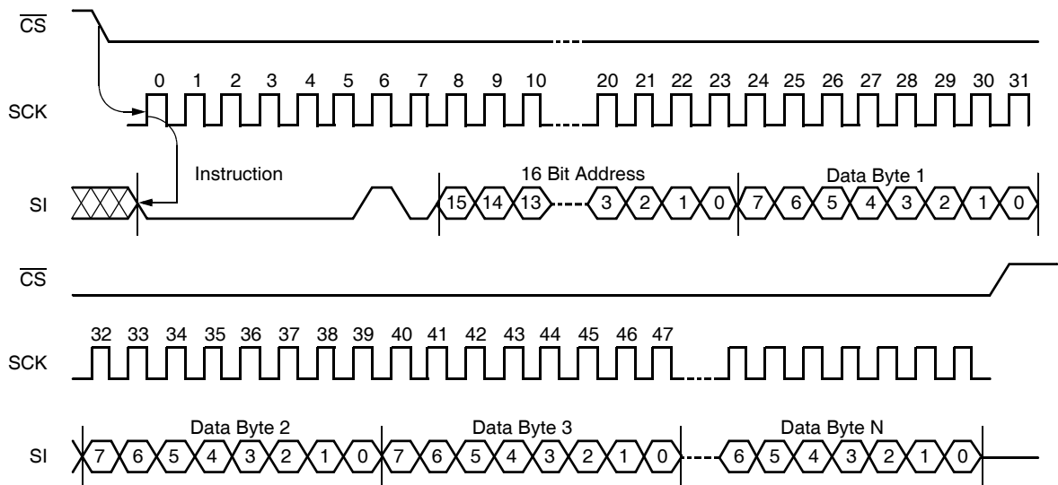
Figure 8. Write Sequence
