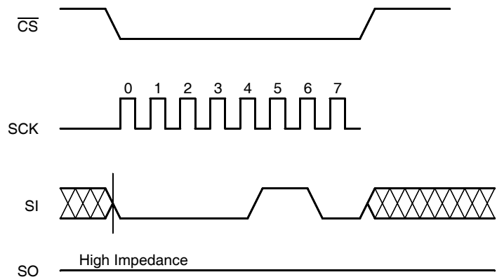
Figure 7. Write Enable Latch Sequence
