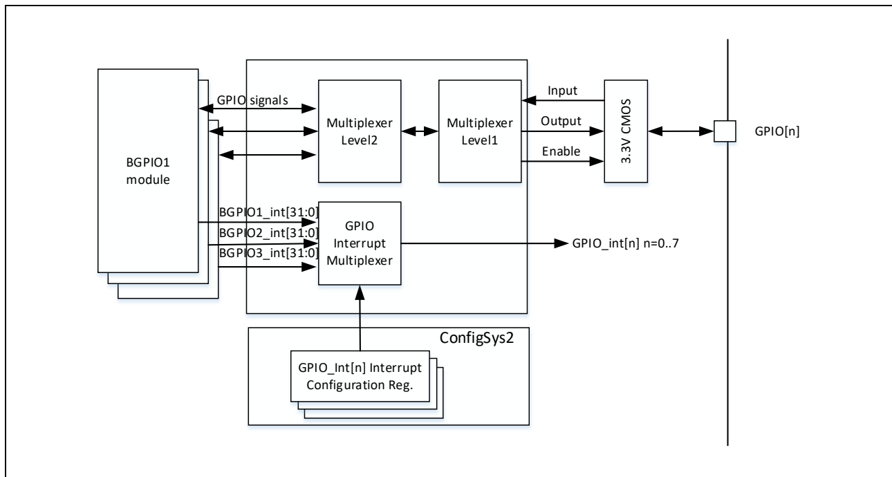
Figure 5.2 GPIO_Int[n] Configuration
