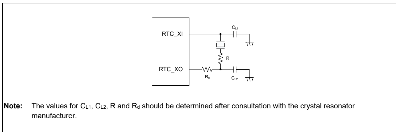
Figure 3.4 Example of Crystal Resonator Connection (RTC)
