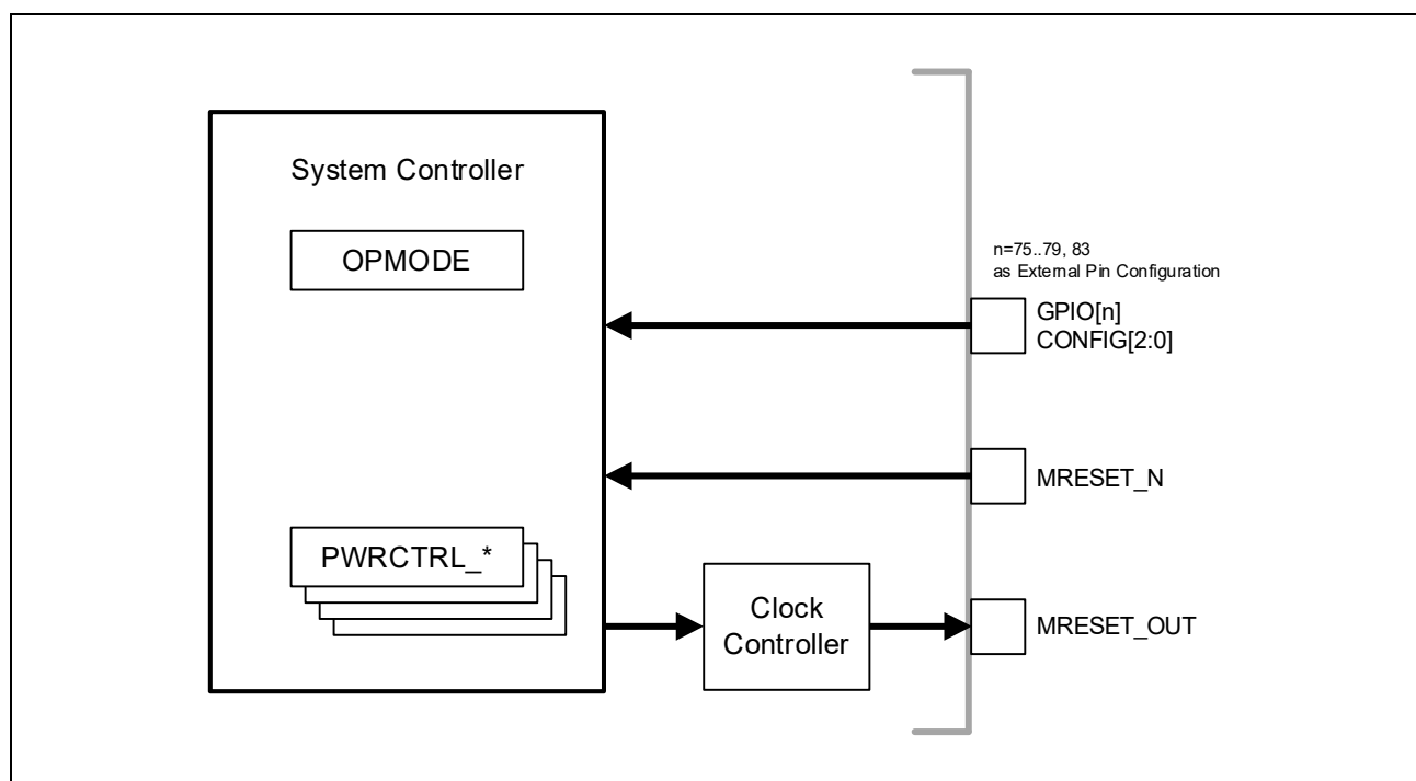
Figure 7.1 System Controller
