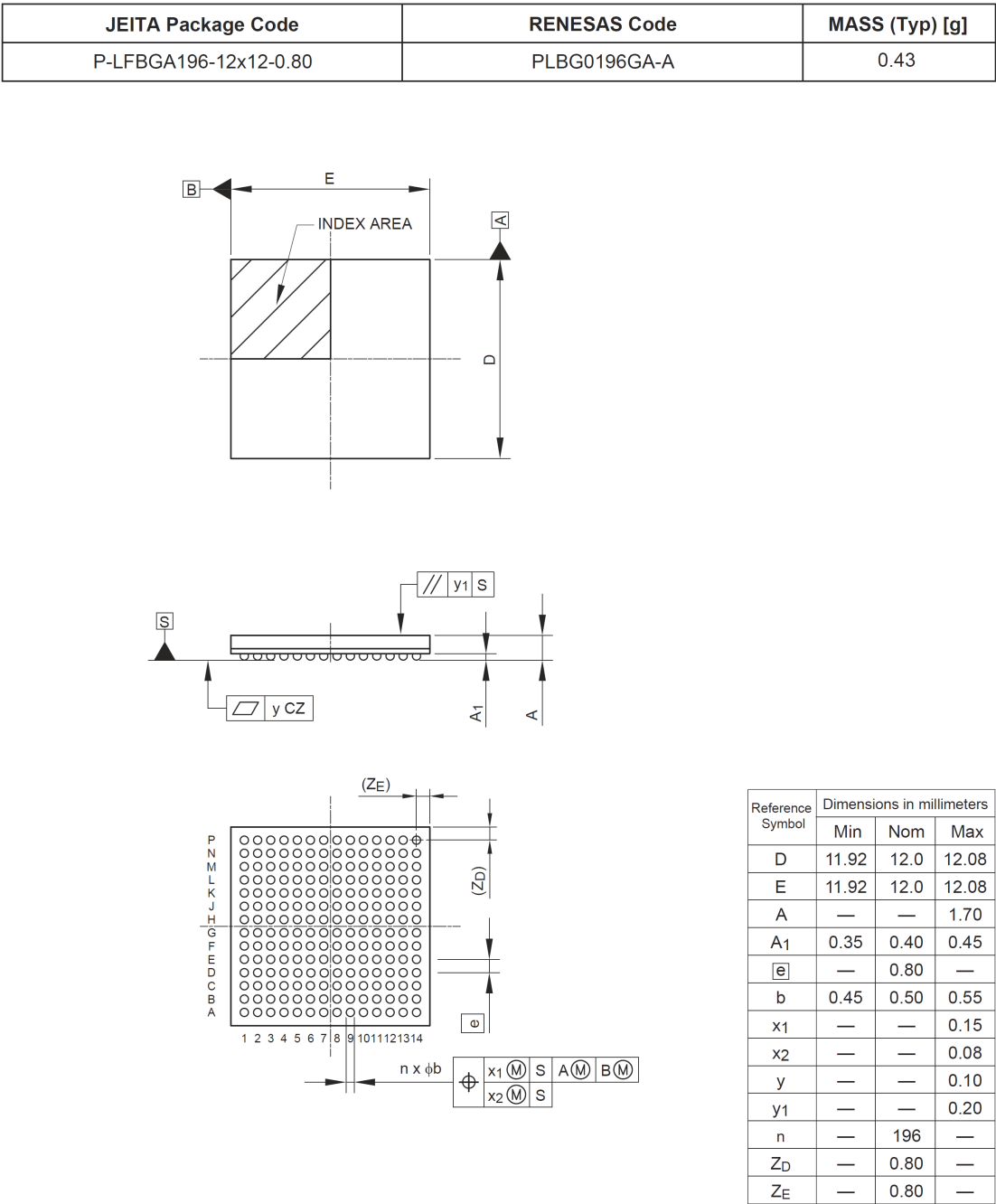
Figure 12.3 BGA-196 Package Dimensions
