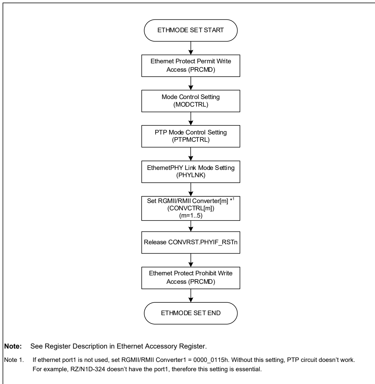
Figure 8.5 ETHMODE_SET Flowchart
