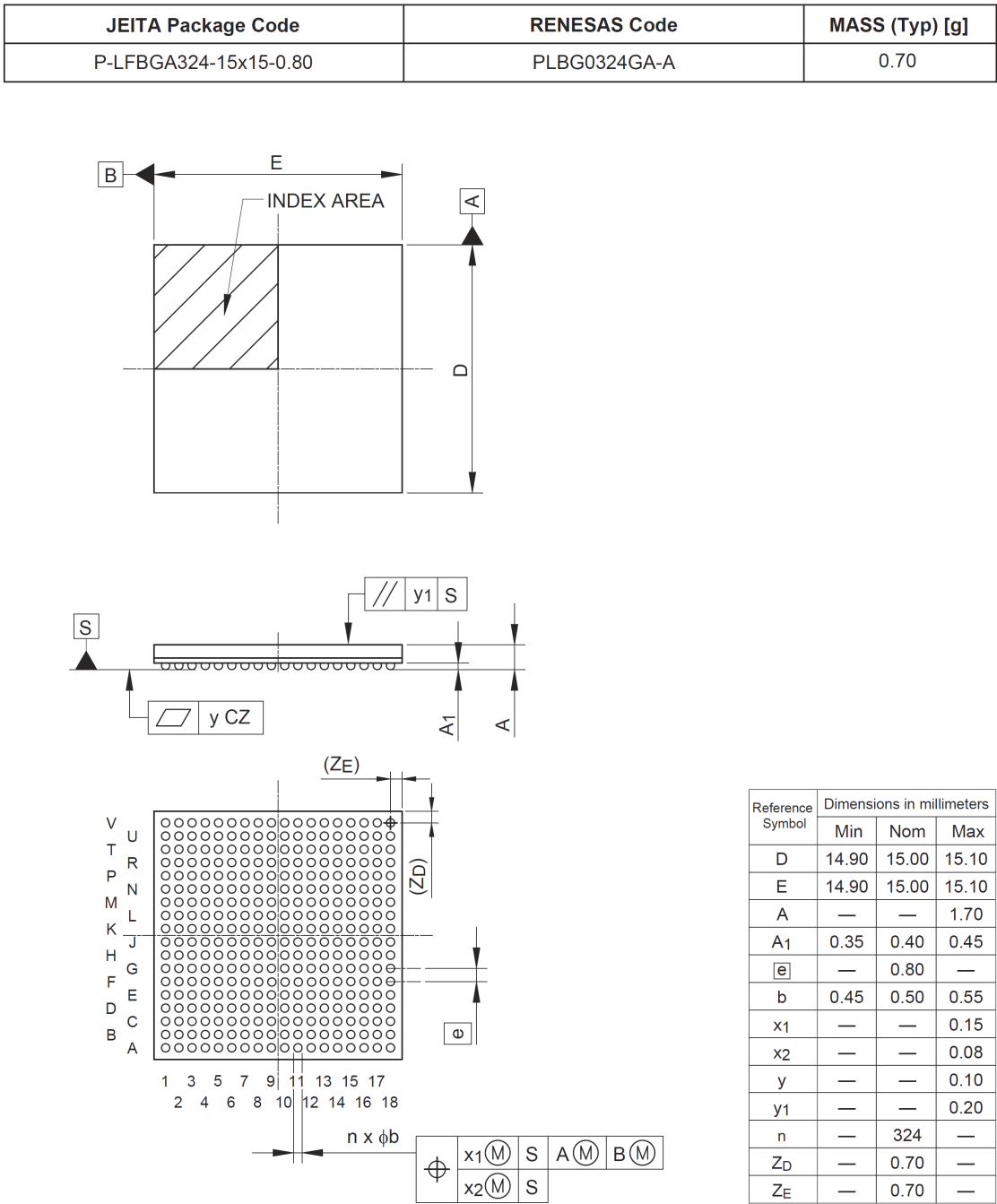
Figure 12.2 BGA-324 Package Dimensions
