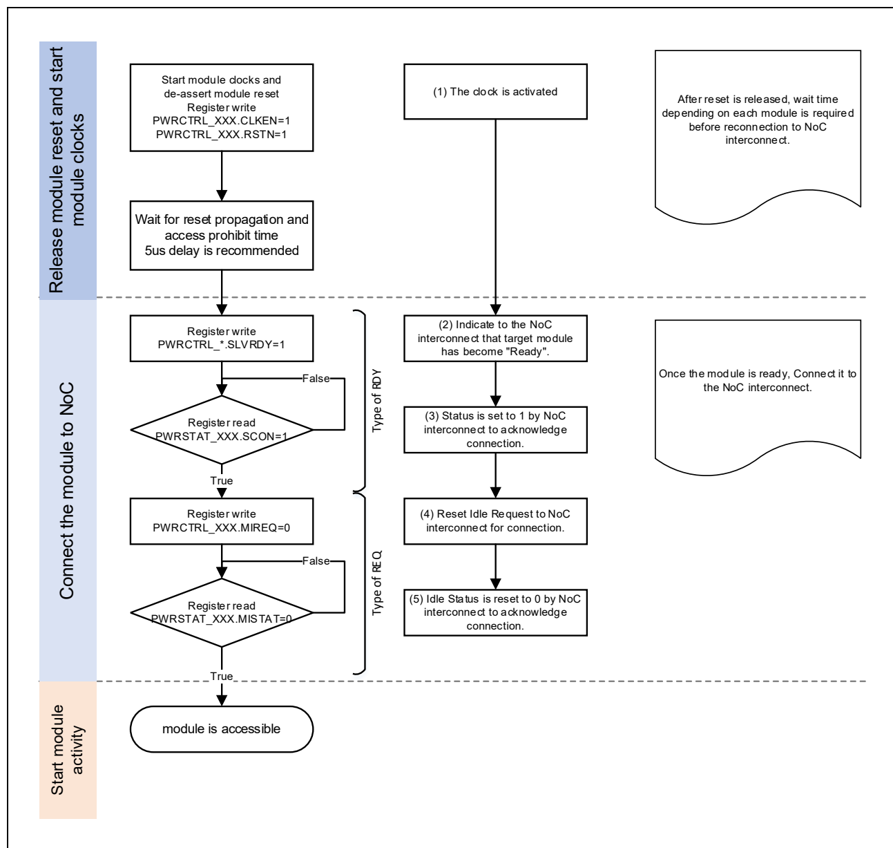
Figure 7.4 Generic Programming Sequence for NoC – Connect
