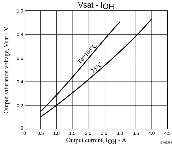
STK672-640B-E Output saturation voltage, V_{sat} - Output current, I_{OH}
