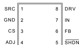
LM PACKAGE (Top View)
