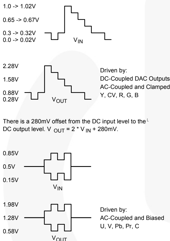
Figure 13. Typical Voltage Levels
