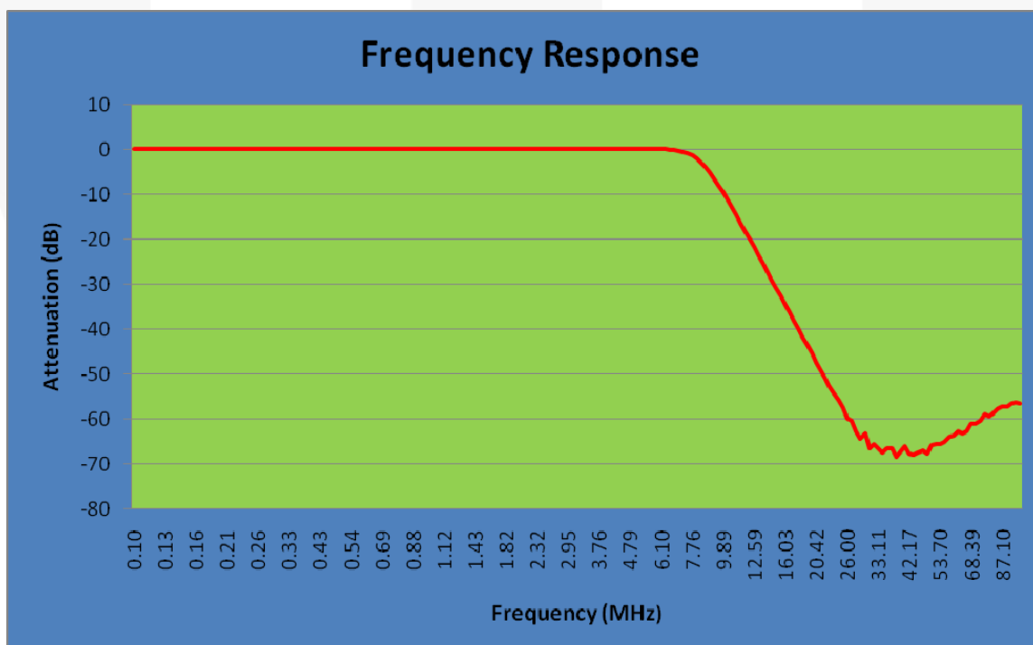
Figure 4. Frequency Response
