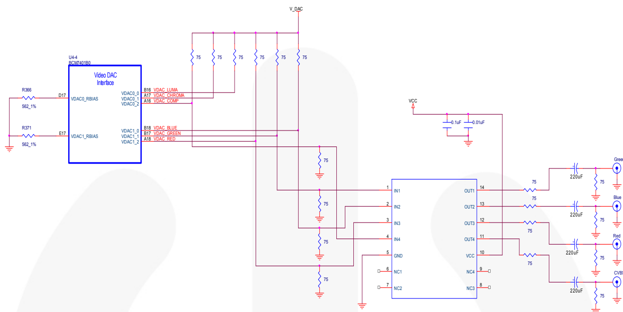
Figure 12. Typical Application
