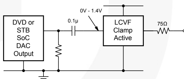
Figure 16. AC-Coupled Inputs, DC-Coupled Outputs
