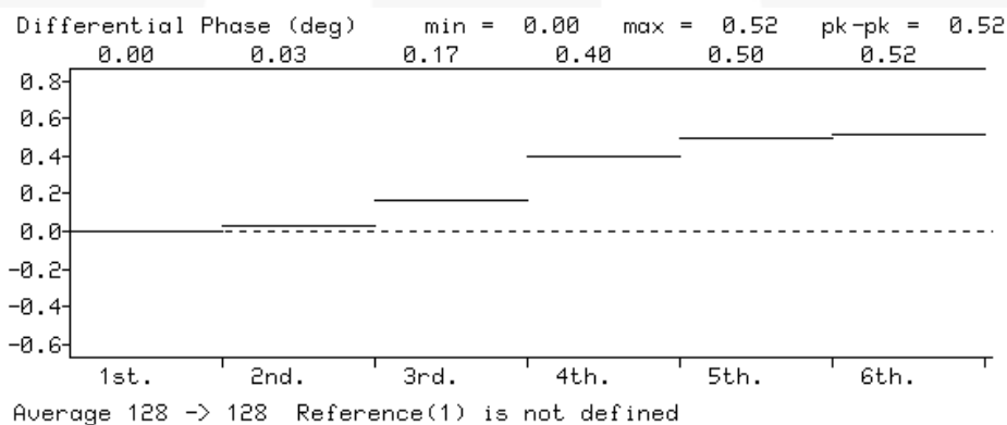
Figure 10. Differential Phase
