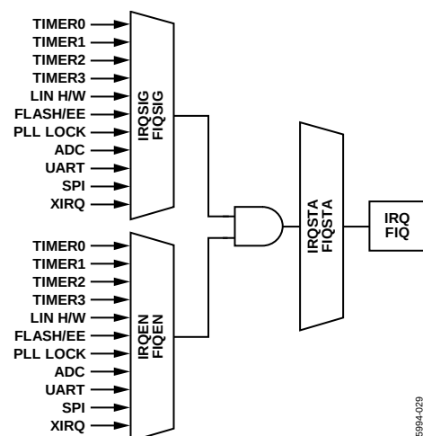
Figure 29. Interrupt Structure
