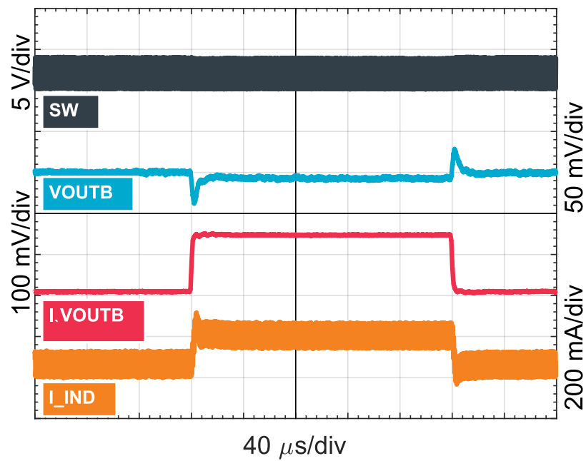
Figure 33: BUCK load transition in PWM mode (MODE=1), I_{\text{out}}=10\text{ mA} \rightarrow 150\text{ mA} \rightarrow 10\text{ mA} (1 \mu\text{s} step), V_{\text{out}}=1.8\text{ V} , V_{\text{BAT}}=3.8\text{ V}
