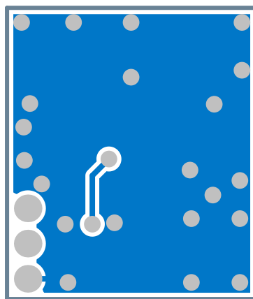
Figure 39: Bottom layer
