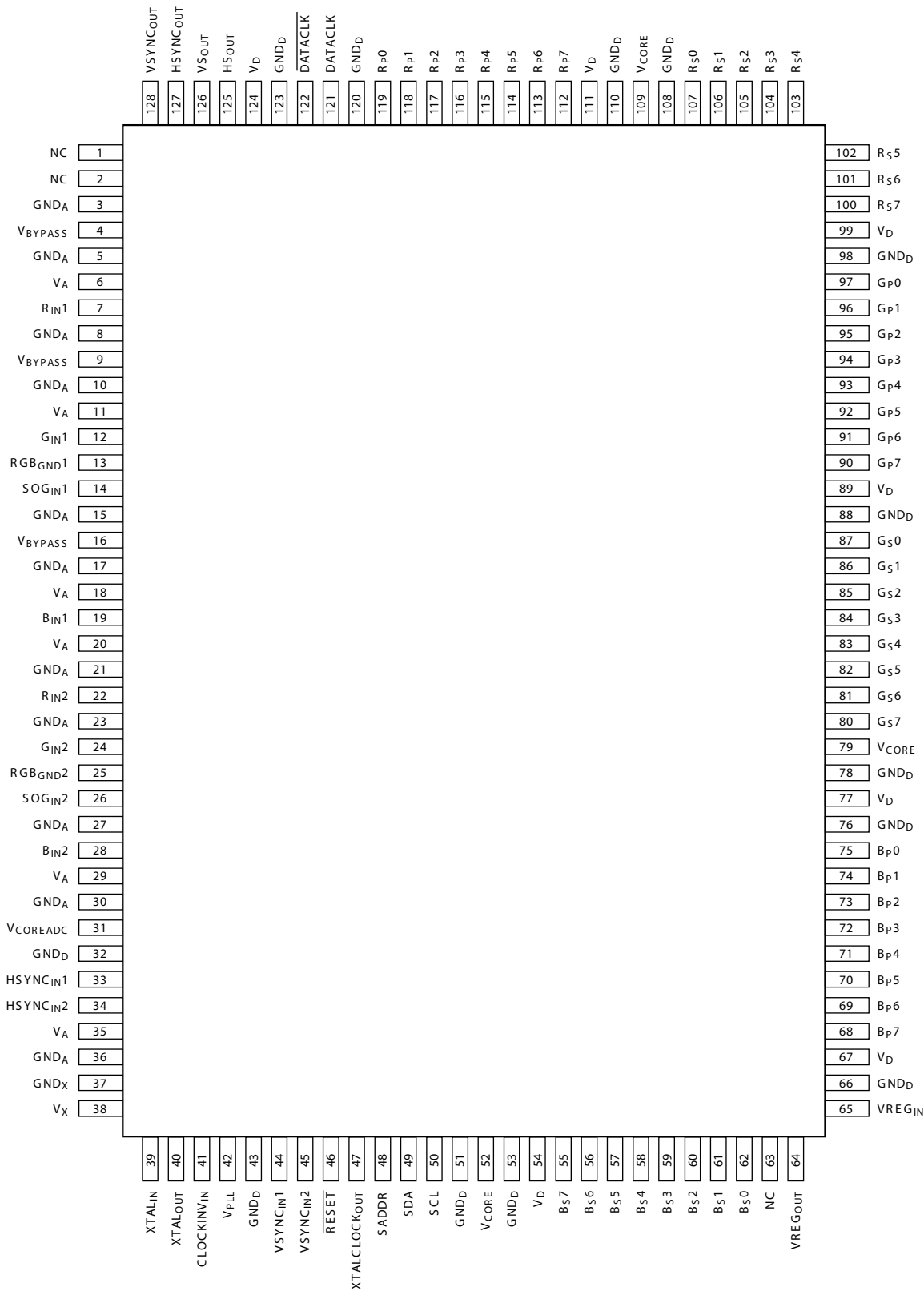
X98014 (128-PIN MQFP) TOP VIEW
