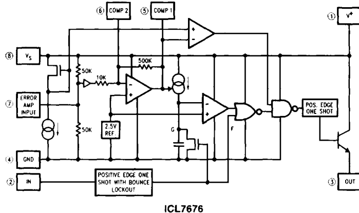
Figure 2: Functional Diagrams
