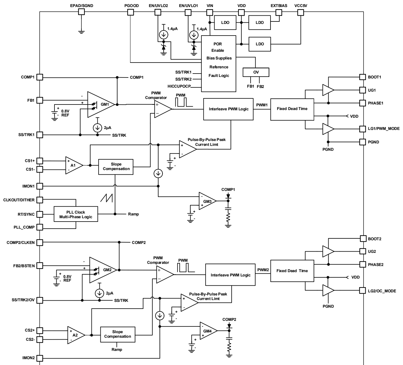
Figure 5. Block Diagram
