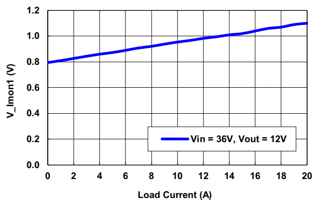
Figure 17. Dual-Phase Output Current I_{OUT} (DC) vs IMON1 Pin Voltage, R_{S\_out} = 4m\Omega , R_{IMON1} = 20k
