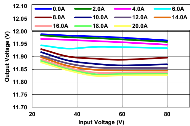
Figure 21. CCM Line Regulation at 25°C
