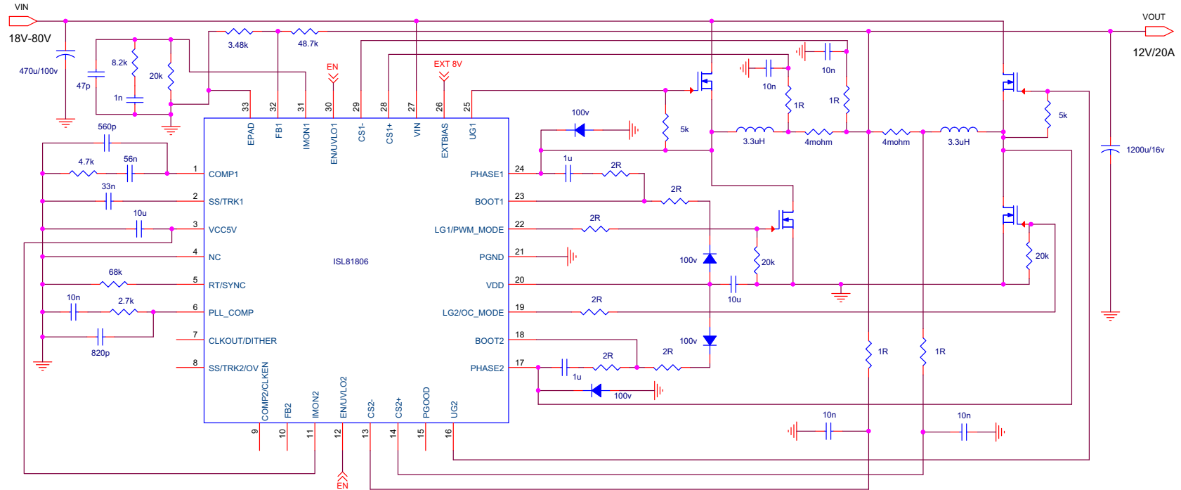
Figure 3. V_{IN} = 18V to 80V , V_{OUT} = 12V , I_{OUT} = 20A Typical Circuit
