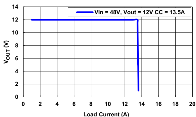
Figure 27. Constant Voltage (CV) and Constant Current (CC) Operation
