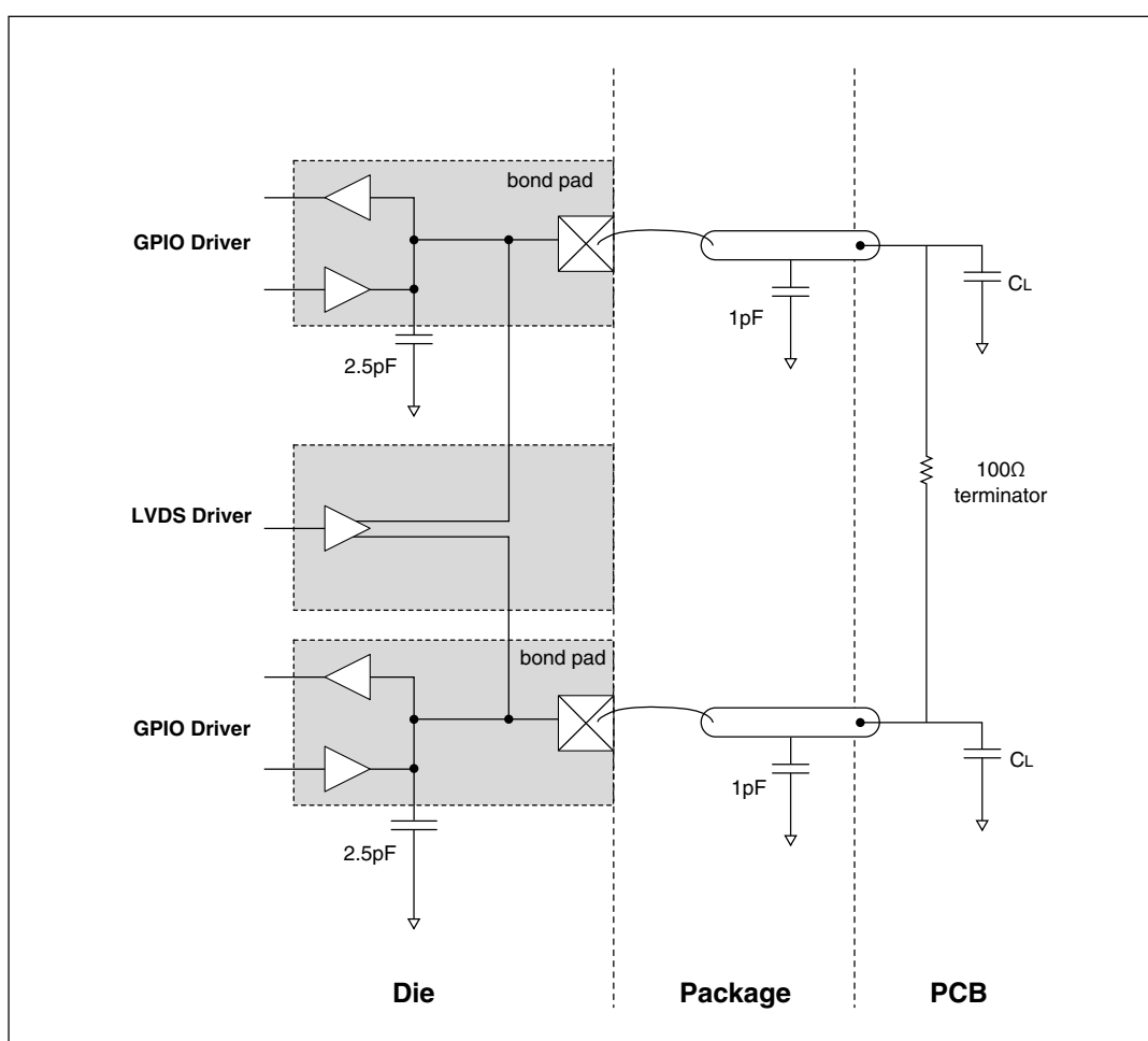
Figure 10. LVDS pad external load diagram
