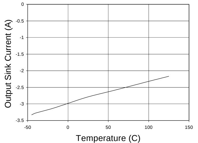
Output Sink Current vs. Temperature V_{\text{SUPPLY}} = 15\text{V}
