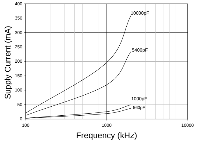
Supply Current vs. Frequency V_{\text{SUPPLY}} = 20\text{V}
