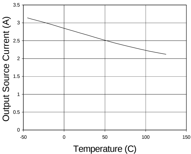
Output Source Current vs. Temperature V_{\text{SUPPLY}} = 15\text{V}
