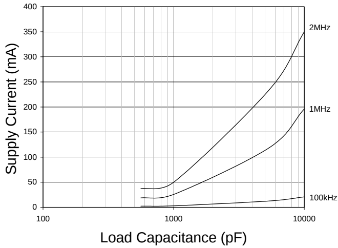
Supply Current vs. Capacitive Load V_{\text{SUPPLY}} = 20\text{V}
