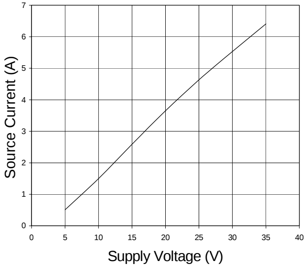
Output Source Current vs. Supply Voltage
