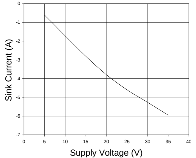
Output Sink Current vs. Supply Voltage
