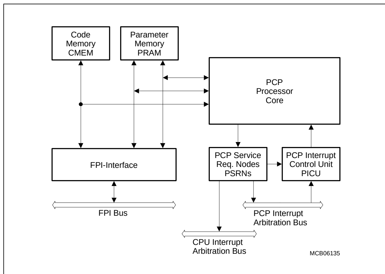
Figure 3-1 PCP2 Block Diagram
