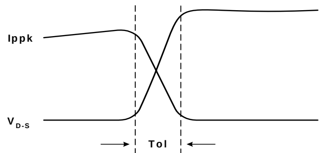
FIGURE 6. SWITCHING CYCLE
