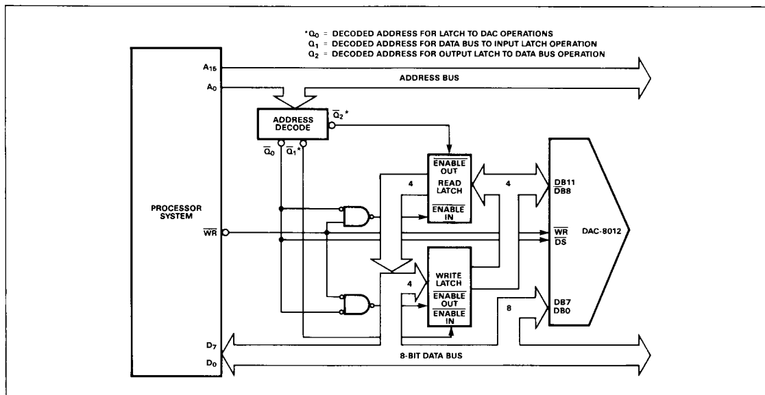
FIGURE 7: 8-Bit Processor to DAC-8012 Interface
