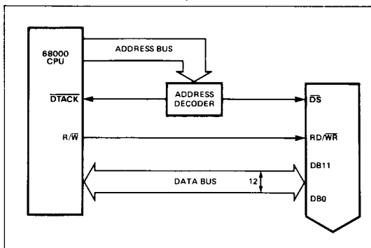
FIGURE 6: 68000 16-Bit Microprocessor to DAC-8012 Interface
