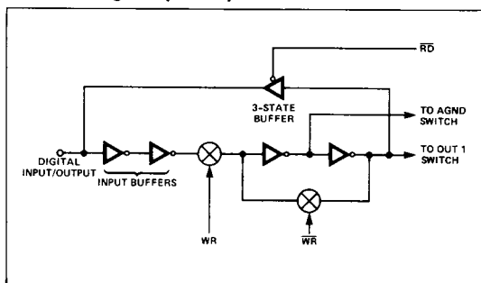
FIGURE 3: Digital Input/Output Structure
