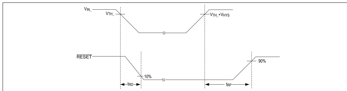
Figure 2. Reset Output Timing
