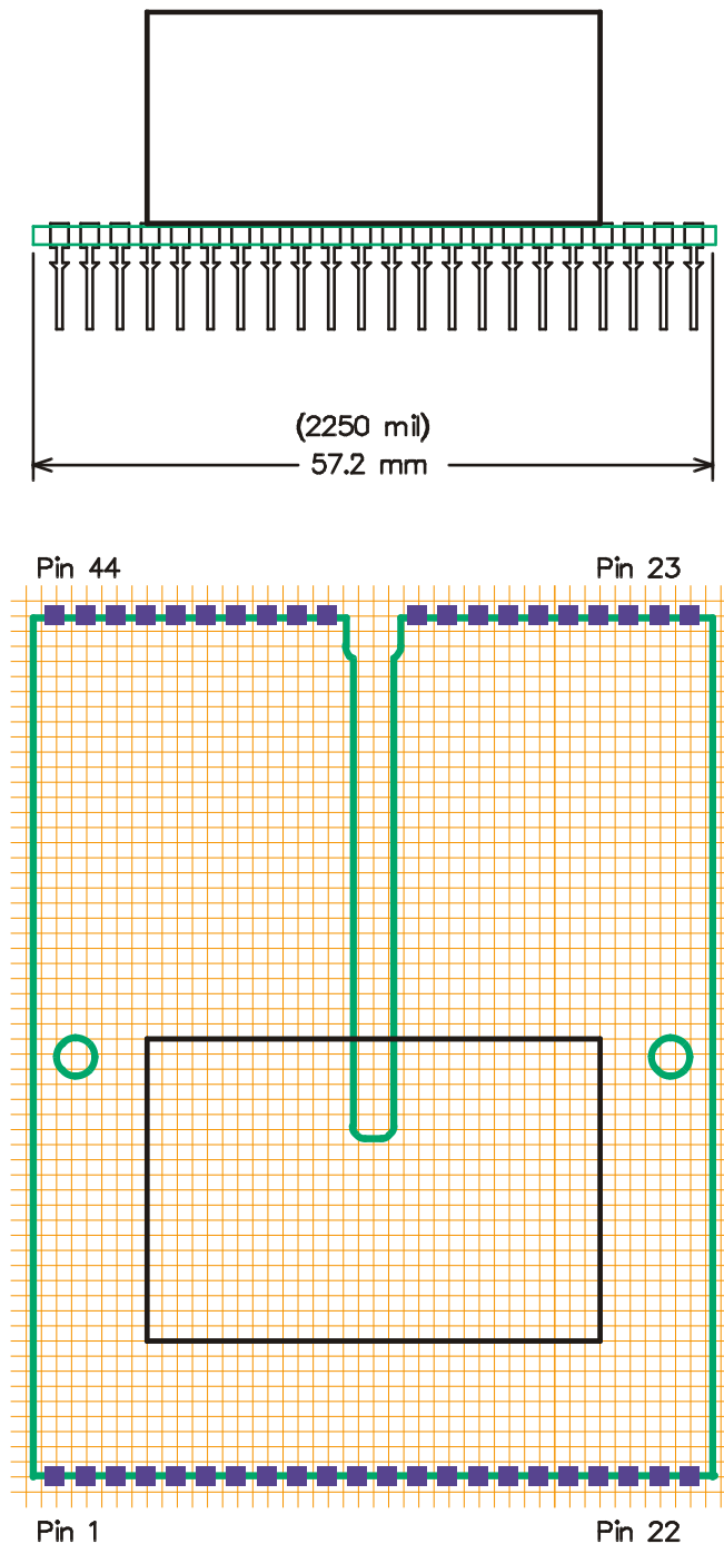
Fig 2 Front view (top) / Layout overview component side (bottom) 2SD315AI-25
