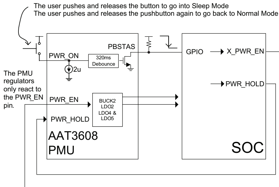
Figure 3: Normal ⇌ Sleep Mode Block Diagram.
