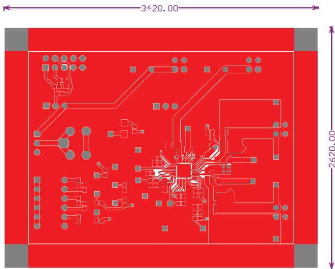
Figure 12: AAT3608 Evaluation Board Top Layer.
