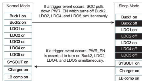
Figure 6: Normal Mode ↔ Sleep Mode Flowchart.
