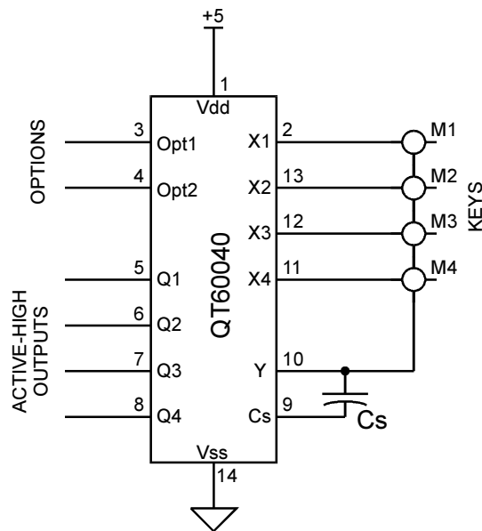
Figure 2-1 Basic Circuit Diagram
