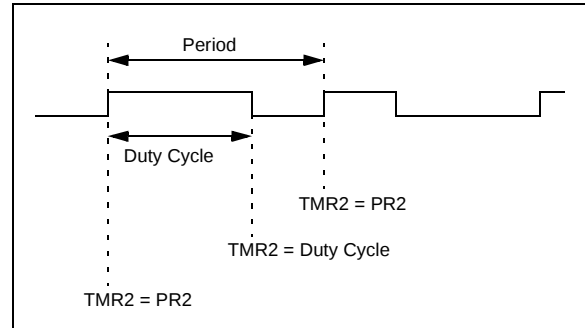
FIGURE 15-2: PWM OUTPUT
