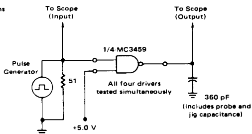
FIGURE 1 — TEST CIRCUIT AND WAVEFORMS FOR PROPAGATION DELAY TIMES
