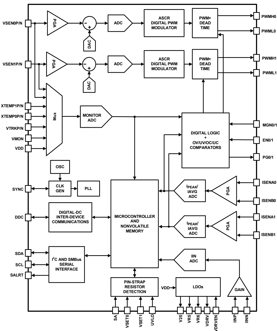
FIGURE 3. BLOCK DIAGRAM
