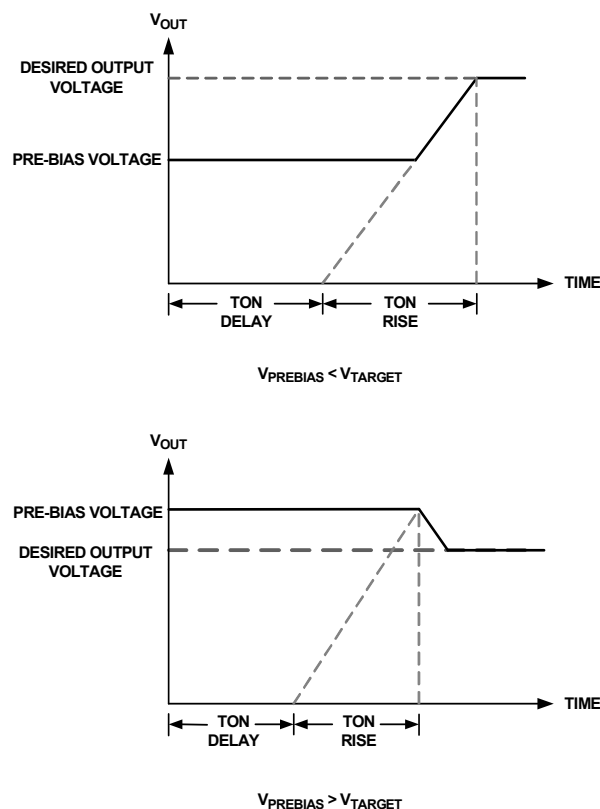
FIGURE 7. OUTPUT RESPONSES TO PREBIAS VOLTAGES
