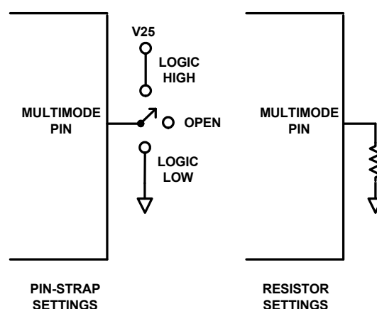
FIGURE 5. PIN-STRAP AND RESISTOR SETTINGS
