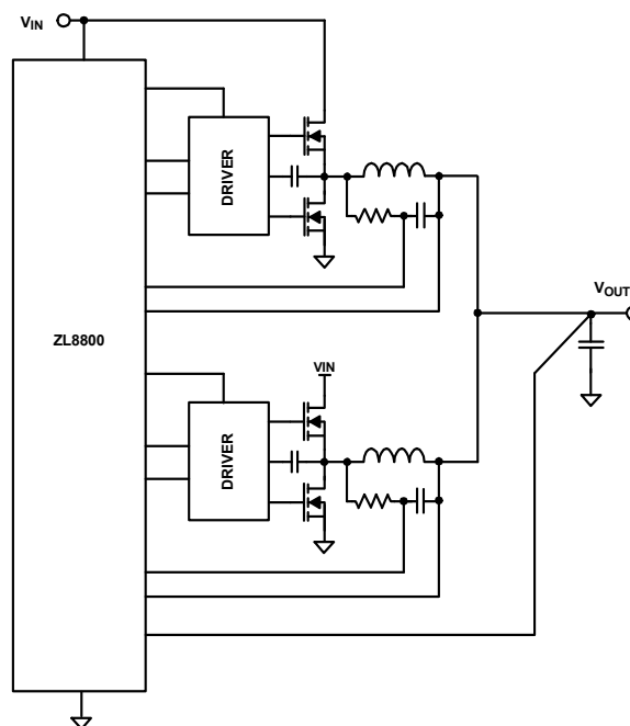
FIGURE 10. DUAL PHASE EXAMPLE
