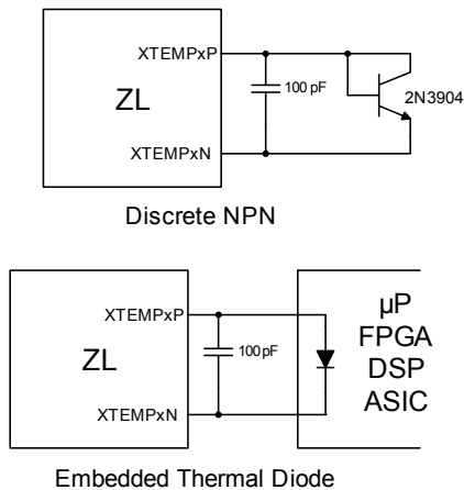
FIGURE 11. EXTERNAL TEMPERATURE MONITORING
